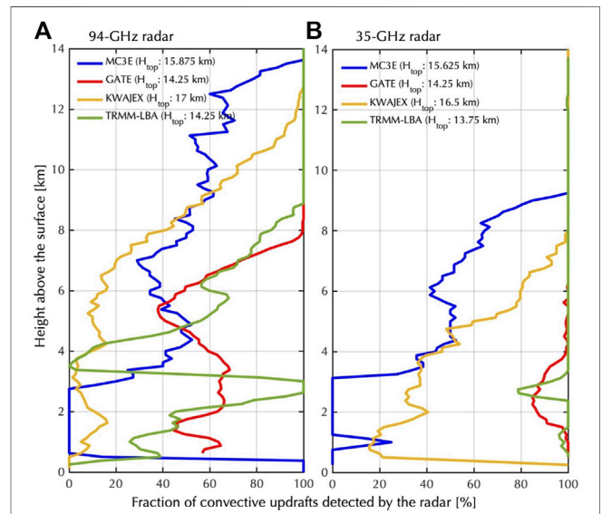
FIGURE 3 | Fraction of convective updraft ( V_{AIR} > 2 \text{ ms}^{-1} ) detected by the (A) 94 GHz and (B) 35 GHz radars as a function of height. An estimate of cloud height ( H_{top} ) for the various cloud types simulated is given in the legend. Results are shown for the different cloud types under study (colors as in Figure 2).
