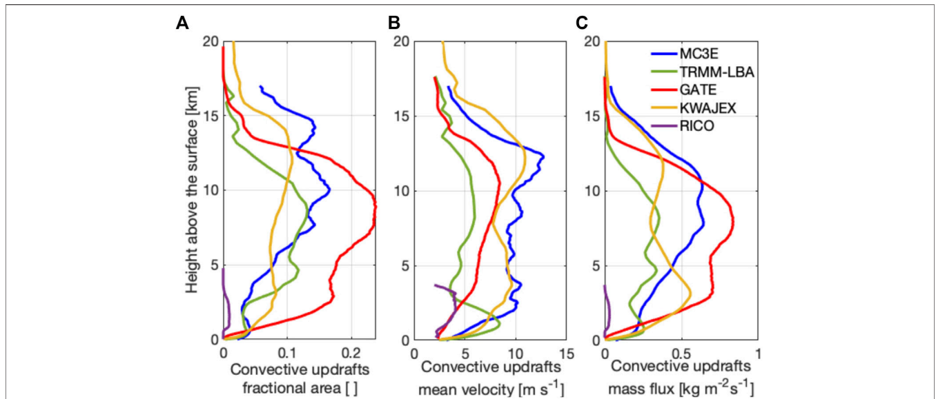
FIGURE 2 | Profiles of storm-averaged convective updraft (A) fractional area, (B) mean velocity, and (C) mass flux estimated directly from the numerical model simulations. Results are shown for the different cloud types under study (MC3E: blue, GATE: red, KWAJEX: yellow, TRMM-LBA: green, RICO: purple).
