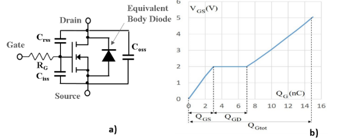
Fig. 2. a) Simplified capacitors model of a GaN HEMT device. b) Gate charge curve at I_D=29A and V_{DS}=40V of the switch device used in the inverter application ( Q_{Gtot}=15nC ).
