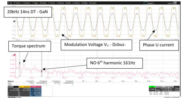
Fig. 9 GaN inverter with 14ns dead time and its effect on torque signal; electrical frequency is 27 Hz, torque 6th harmonic is null
