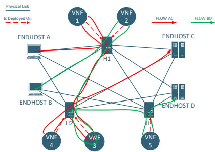
FIGURE 5. Physical Flow Mapping Example
