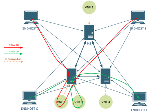
FIGURE 12. Overlapping Flows Example
