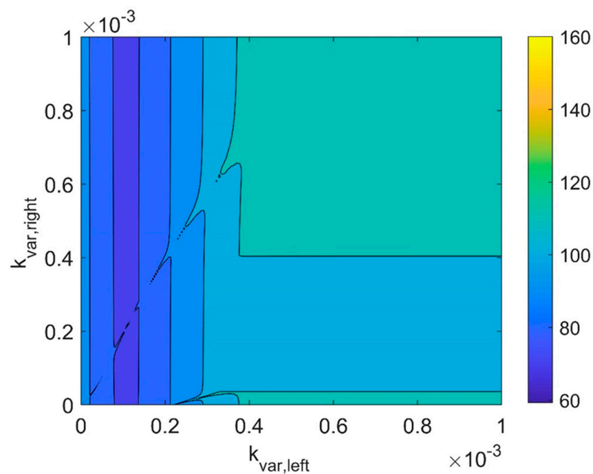
Figure 15. Objective function for a variation of k_{var,left} and k_{var,right} in the range between 0 and 1 \times 10^{-3} .
