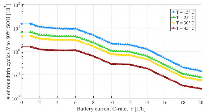
Figure 1. Number of allowed battery roundtrip cycles as function of the C-rate and temperature as predicted by the implemented ageing model.
