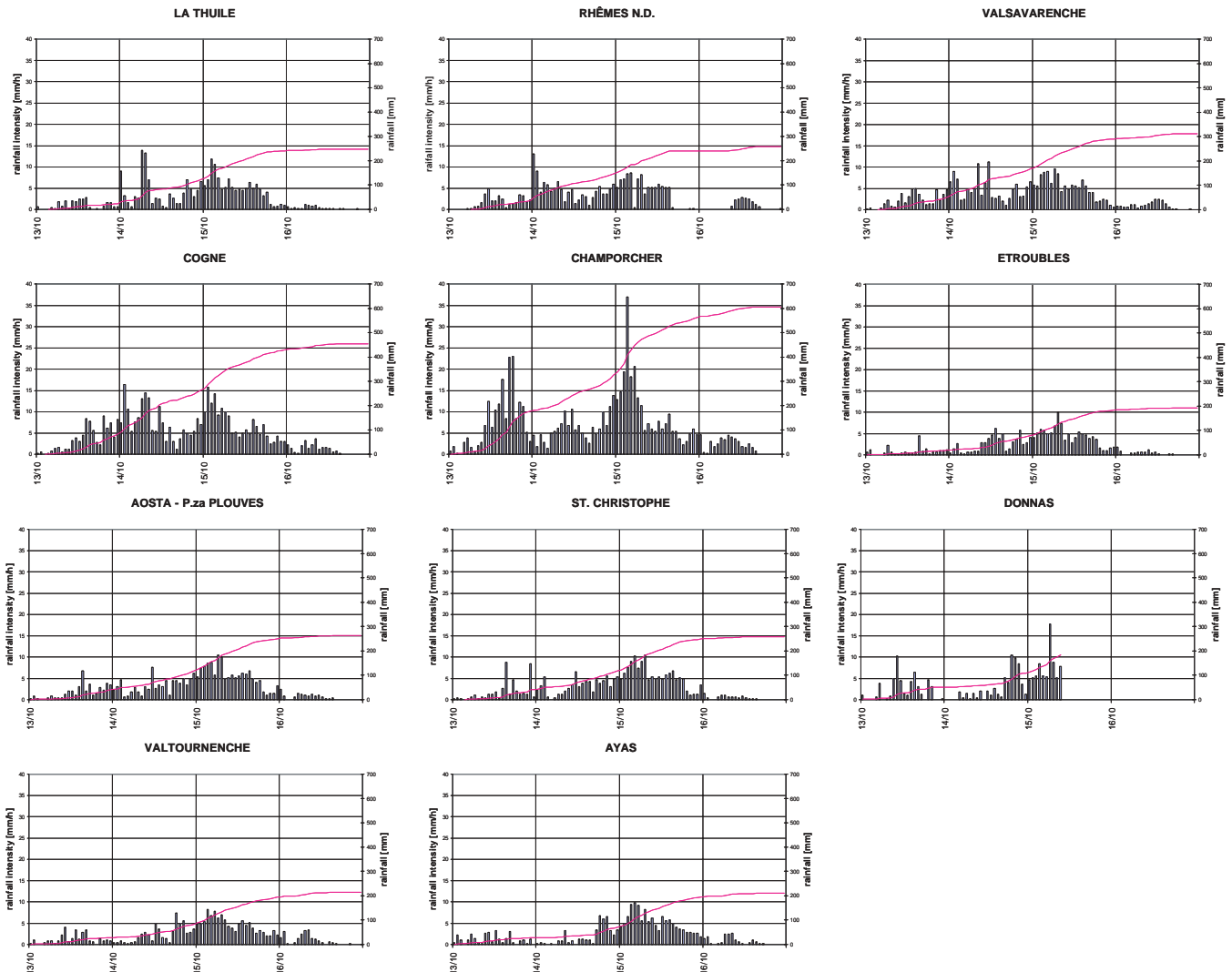
Figure 5 Pluviograms.
