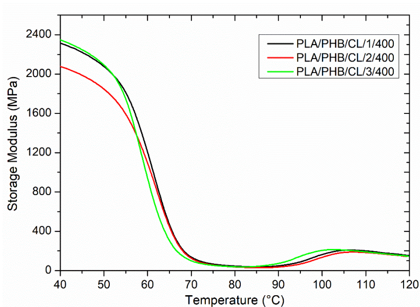
Figure 117. DMA traces for filled blend processed with different screw profiles and unfilled blend. Reprinted under CC BY 4.0 license from [221].
