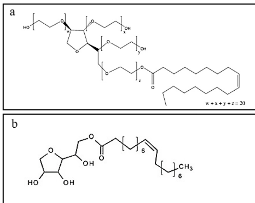
Figure 62. Chemical structures of Tween (a) and Span (b) non-ionic liquid surfactants.
