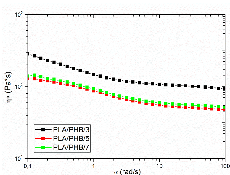
Figure 102. Complex viscosity \eta^* of blends PLA/PHB processed with different flow rates.
