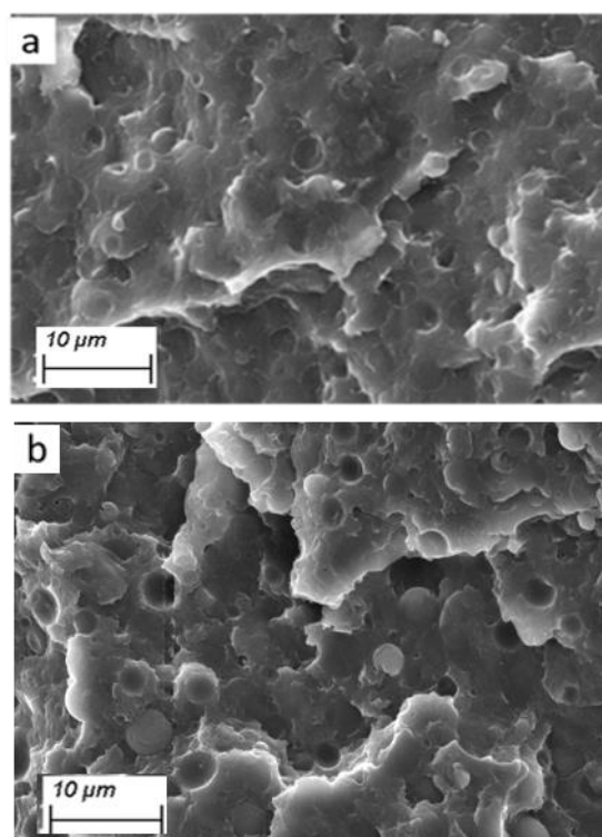
Figure 104. SEM micrographs of PLA/PHB blends processed at 3 kg/h (a) and 5 kg/h (b).
