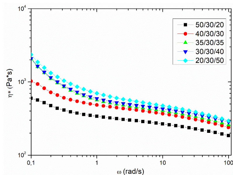
Figure 135. Complex viscosity \eta^* of PLA/PBS/PHBt polymer blends.
