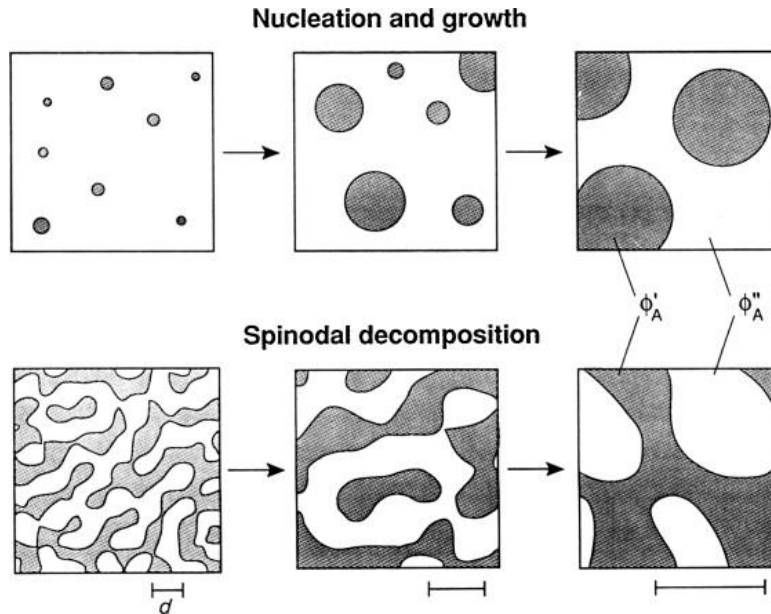
Figure 6. Nucleation and growth NG and spinodal decomposition SD patterns in a binary polymer blend. Reprinted with the permission of [20].
