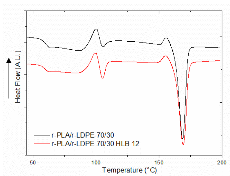
Figure 75. DSC thermograms of non-compatible and compatibilized r-PLA/r-LDPE 70/30 blends; recorded during second heating ramp. Reprinted with the permission from [189].
