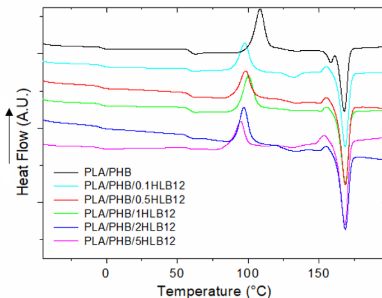
Figure 82. DSC thermograms for non-compatible blend and HLB12-containing systems (second heating scan). Reprinted under CC BY 4.0 license from [190].
