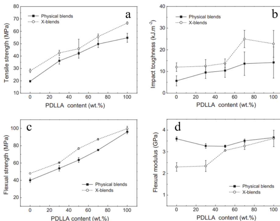
Figure 36. Effect of PDLLA content on the mechanical properties of the PHB/PDLLA blends before and after partial crosslinking by using 0.5 wt% DCP: tensile strength (a), notched Izod impact toughness (b), flexural strength (c) and flexural modulus (d). Modified from [124].
