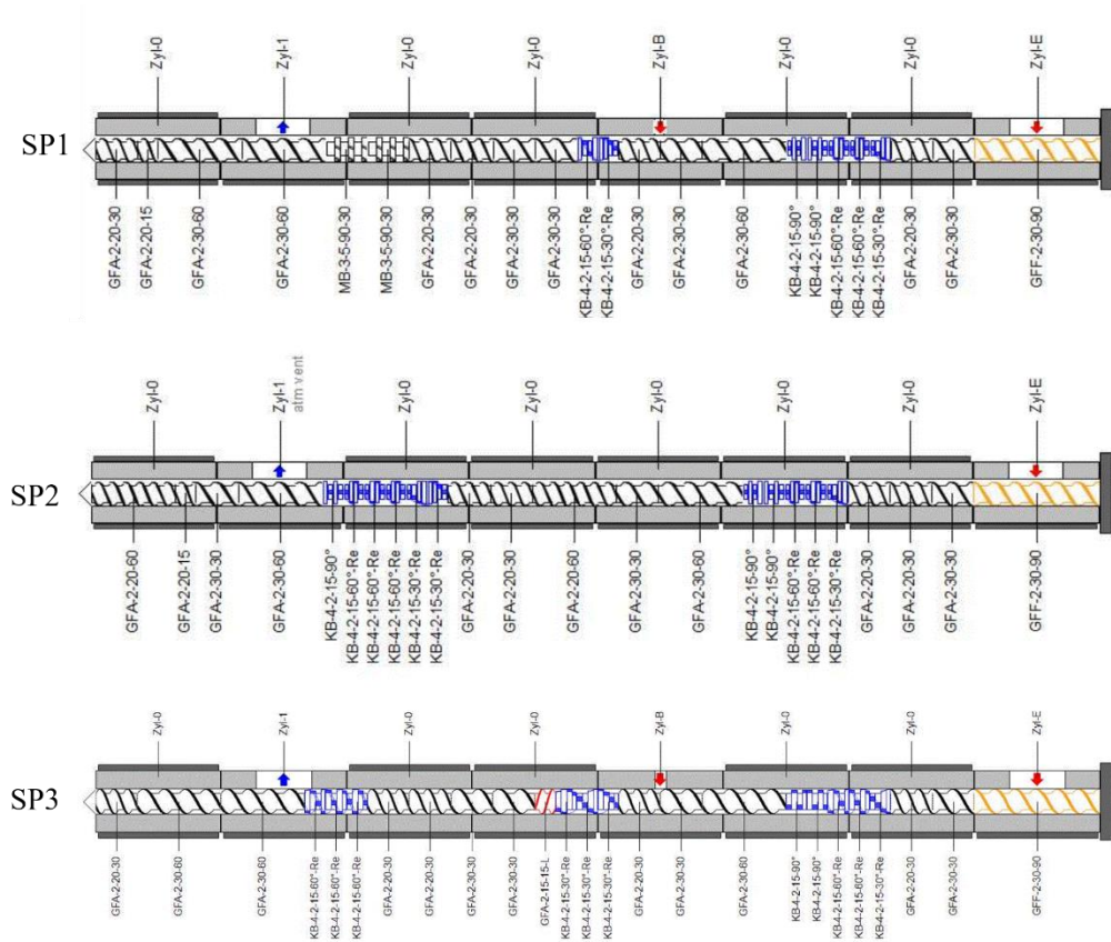
Figure 95. Screw configurations for PLA/PHB process (3 kg/h and 400 rpm).
