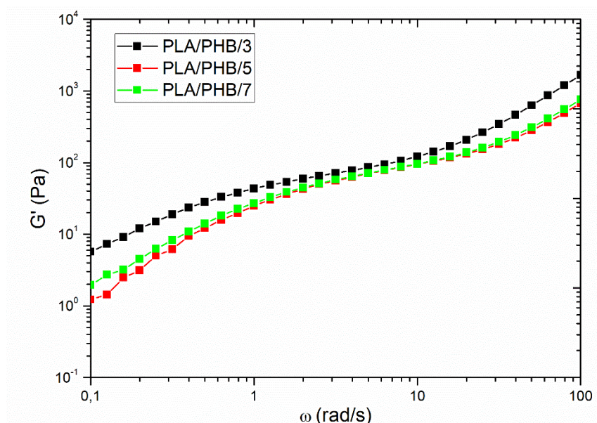
Figure 103. Storage modulus G' of blends PLA/PHB processed with different flow rates.
