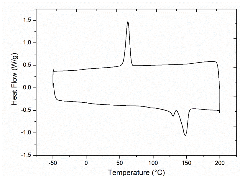
Figure 132. DSC traces recorded during cooling and second heating ramp of PHBt.
