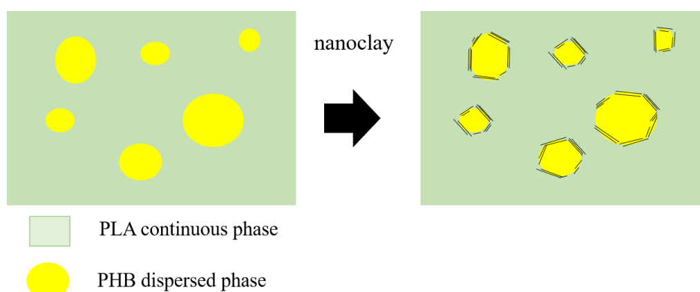
Figure 108. Schematic representation of the localization fillers at the interface between PLA and PHB.
