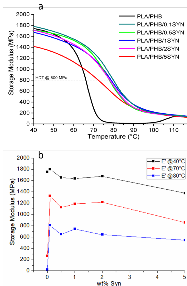
Figure 85. DMA traces for Syn-containing systems (a) and trend of Storage modulus E' as a function of Syn content in the PLA/PHB blends at different temperatures (b). Modified under CC BY 4.0 license from [190].
