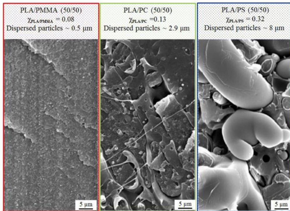
Figure 21. Interaction parameter and morphologies of PLA/PMMA, PLA/PC and PLA/PS. All the formulations are at 50wt%/50 wt%. The interaction parameters were calculated using the solubility parameters of the components. Reprinted with the permission from [52].
