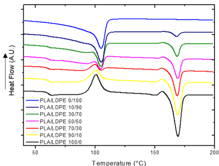
Figure 66. DSC thermograms of non-compatible PLA/LDPE blends, recorded during the second heating scan. Reprinted with the permission from [189].
