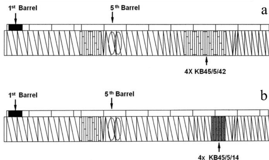
Figure 58. Type screw 4KB45/5/42 with four KB45/5/42 kneading blocks in the mixing region (a). Type screw 4KB/45/5/14 with four KB45/5/14 kneading blocks in the mixing region (b). Both screws have two kneading blocks type KB45/5/42 before the side feeder in the 5th barrel. Reprinted with the permission from [187].
