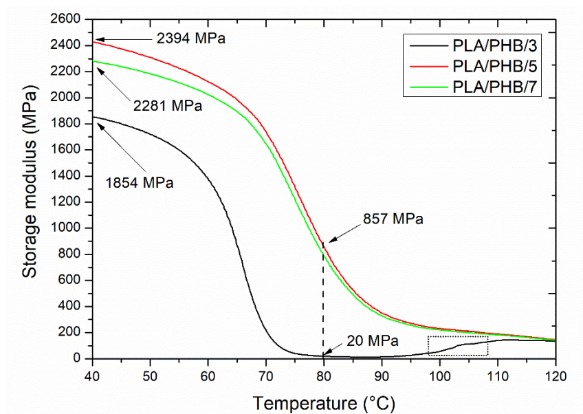
Figure 105. Storage dynamic modulus E' of blends PLA/PHB processed with different flow rates.
