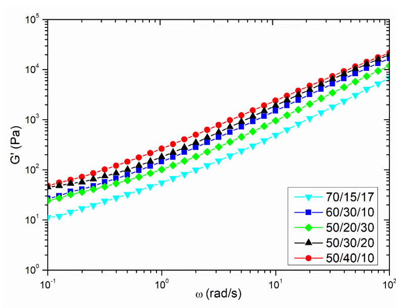
Figure 125. G' trends of PLA/PBS/PHB polymer blends.
