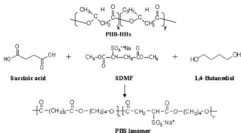
Figure 41. Structure of PHB-HHx and PBS ionomer. Reprinted with the permission from [144].
