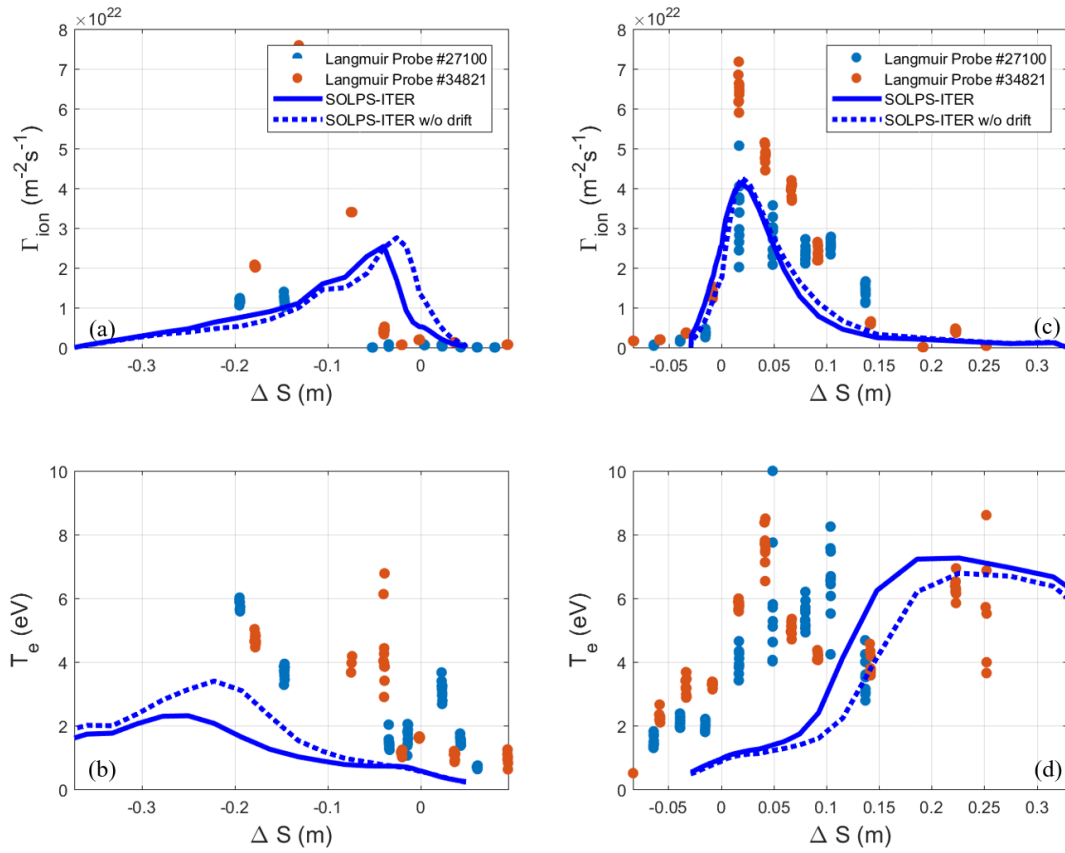
Figure 6. Comparison between measured and modeled value of (a) ion flux \Gamma_{ion} at the inner target, (b) electron temperature T_e at the inner target, (c) ion flux \Gamma_{ion} at the outer target, (d) electron temperature T_e at the outer target for the complete detachment state. For experimental data, both discharge #27100 and #34821 are presented. Solid lines are for cases with drifts, and dash lines are for cases without drift.
