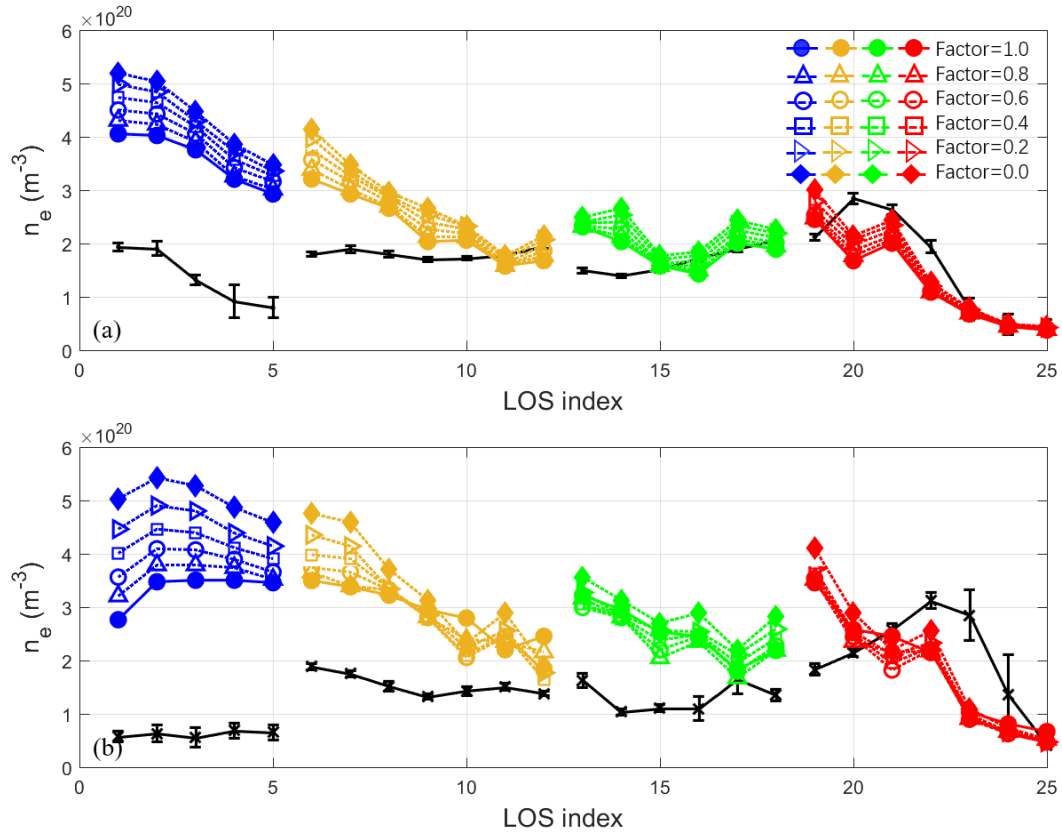
Figure 12. Modelled and measured electron densities n_{e,inner} along LOS for (a) the fluctuating detachment state and (b) the complete detachment state.
