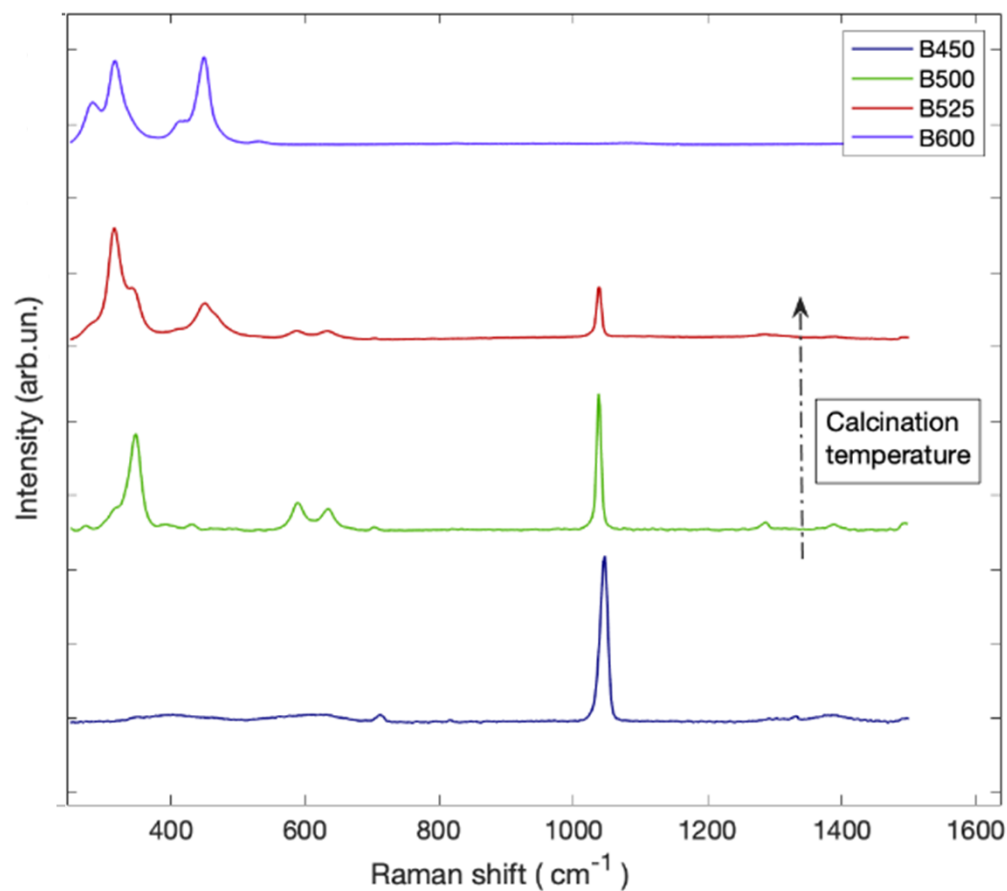
Figure 1. Raman spectra of the synthesized materials. From bottom to top: B450, B500, B525, B600.
