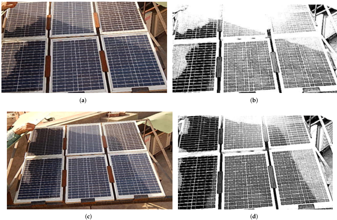
Figure 6. Image processing techniques in the MATLAB libraries. (a) Partial shading case 1, Actual image. (b) Case 1, Processed image. (c) Partial shading case 2, Actual image. (d) Case 2, Processed image.
