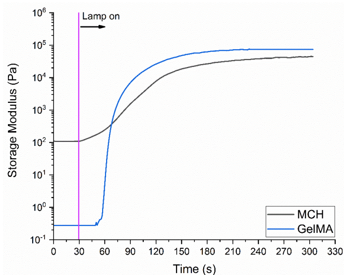
Figure 4. Photoreology curves recorded for the MCH formulation (3 wt% solubilized in acetic acid-water solution containing 2 phr of Irgacure 2959), GelMA formulation (10 wt% solubilized in distilled water containing 1 phr of Irgacure 2959).
