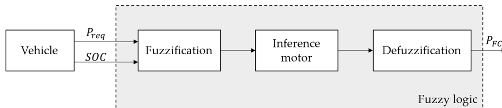
Figure 6. General architecture of the fuzzy logic controller.
