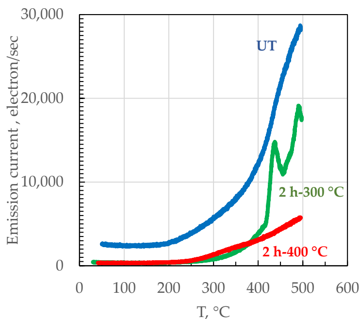
Figure 3. Exo-electron emission (EEE) of the AlSi10Mg LPBF specimens after different post heat treatments as a function of temperature (XZ-specimens).
