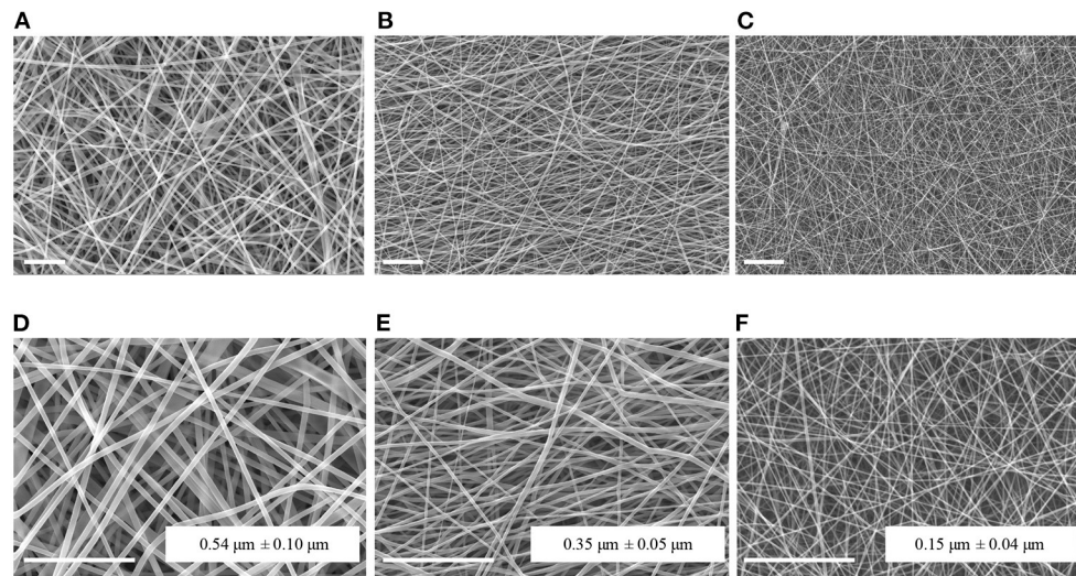
FIGURE 1 | SEM micrographs and average fiber diameters of PCL ( A,D ), Gel ( B,E ), and PCL-Gel ( C,F ) nanofibers at different magnifications ( A–C : 2kx; D–F : 5kx). Scale bars equal to 10 \mu\text{m} .
