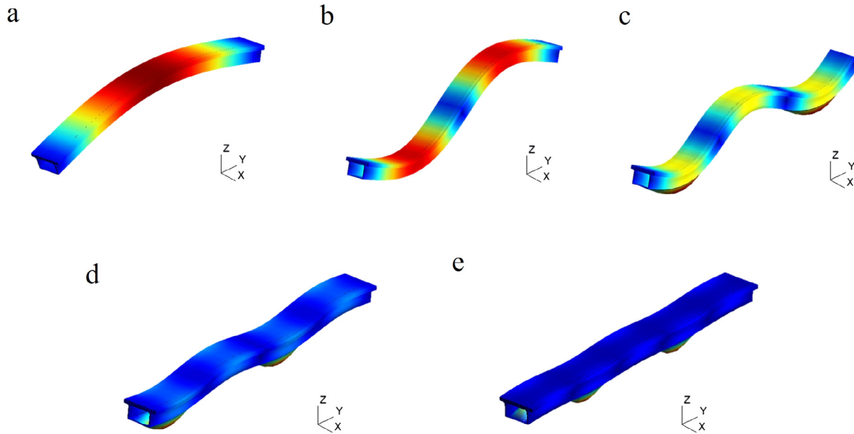
Fig. 6. First modes related to m = 1 - 5 of Box-girder cross-section by the 36L9 model. (a) m = 1, f = 15.19 Hz; (b) m = 2, f = 57.80 Hz; (c) m = 3, f = 118.74 Hz; (d) m = 4, f = 175.19 Hz; (e) m = 5, f = 198.02 Hz.
