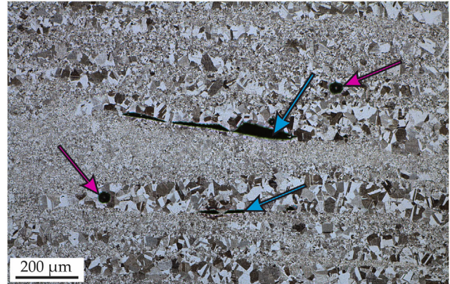
Figure 4. Visible light microscopy image of the occurring porosities in EBM Ti-48Al-2Cr-2Nb. Whereas spherical pores stem from Ar-entrapment (magenta arrows), elongated pores between adjacent powder layers form due to unfavorable process parameters (blue arrows). This lack of fusion porosity exclusively appears below the large \gamma -grain bands, which, therefore, represents the non-Al-depleted zones toward the bottom of melt baths. The building direction is upwards.
