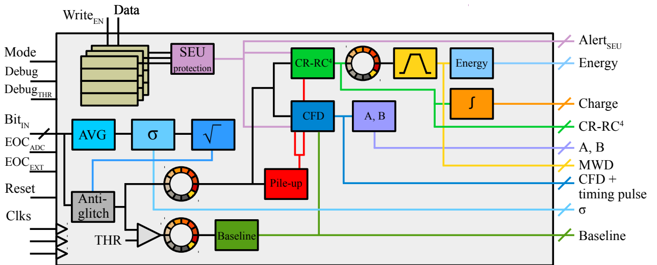
Figure 4.3: Digital signal processor architecture.
