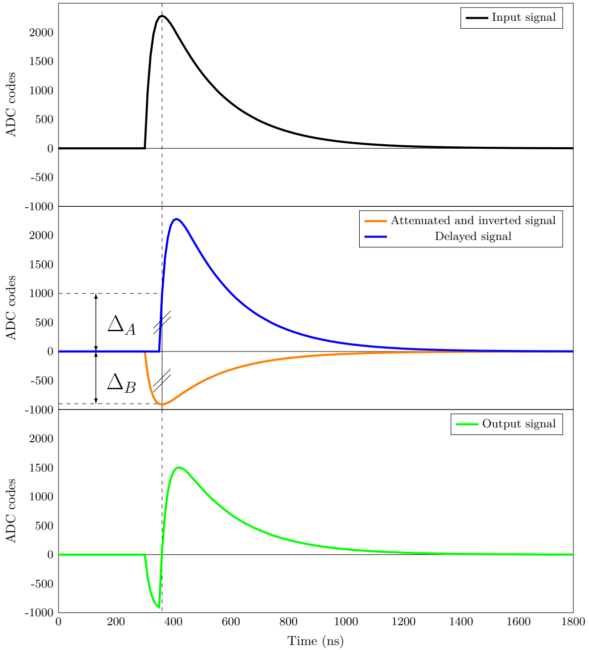
Figure 4.30: The constant fraction method (ideal case).
