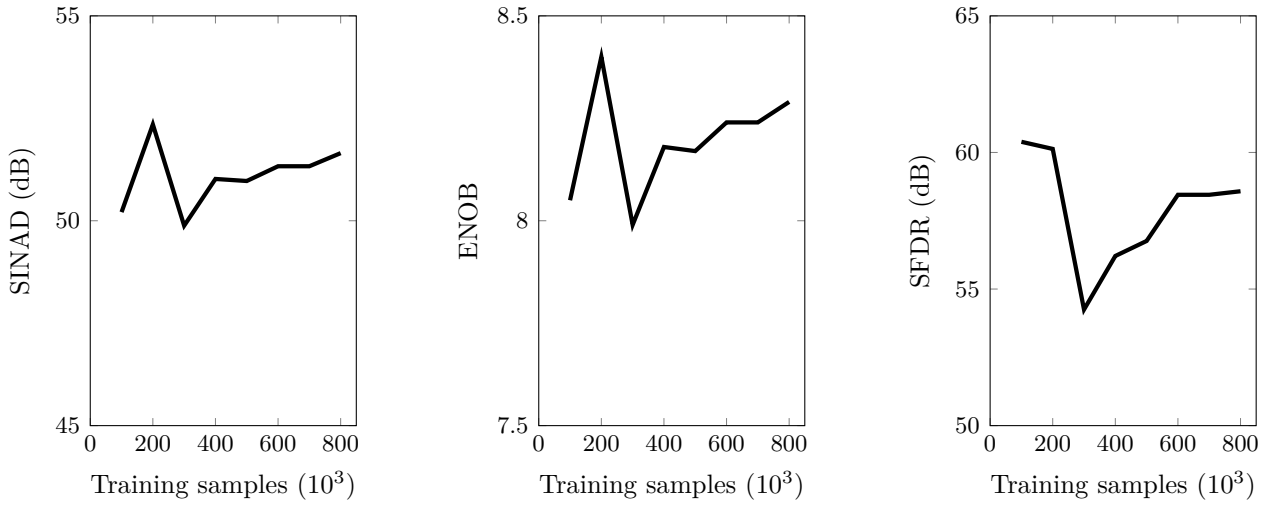
Figure 5.12: Figures of merit outcomes for different numbers of training samples using a ramp signal as input.
