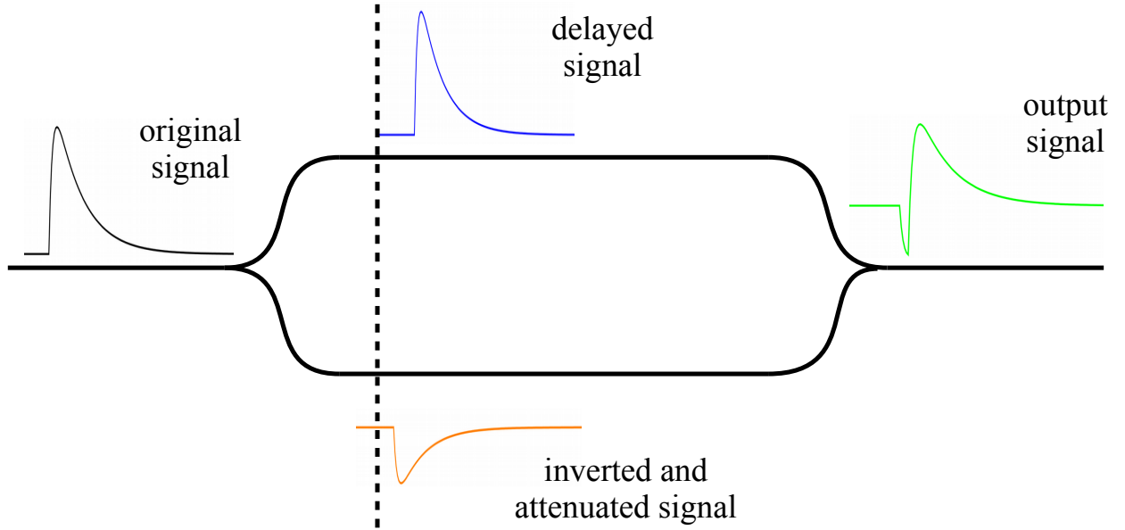
Figure 4.29: CFD algorithm
