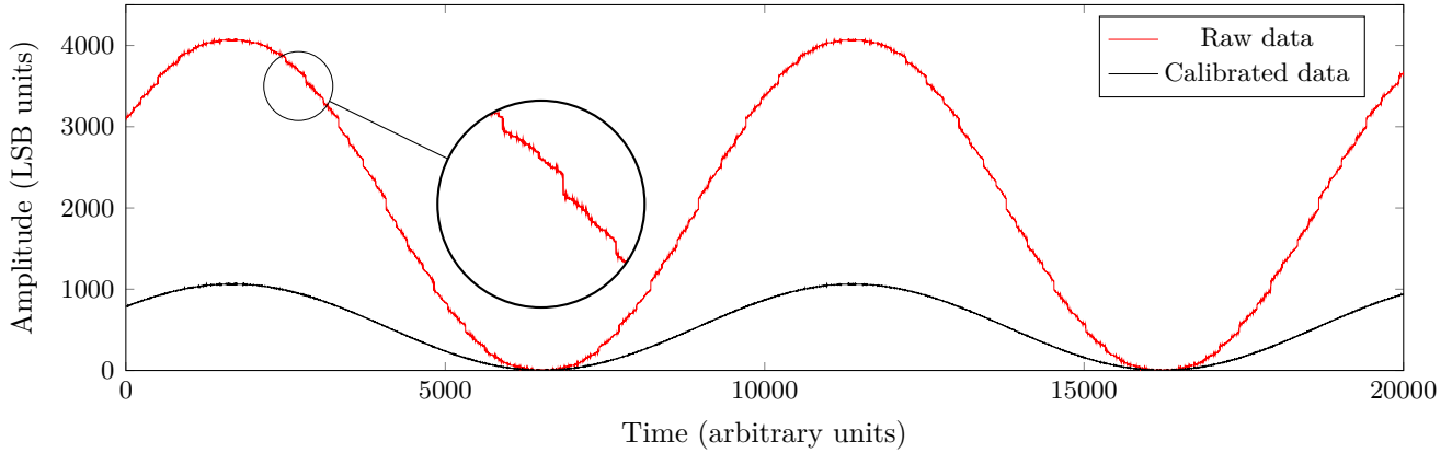
Figure 5.8: The two sinusoidal signals before the calibration (red) and after the correction (black) obtained from the sperimental setup.
