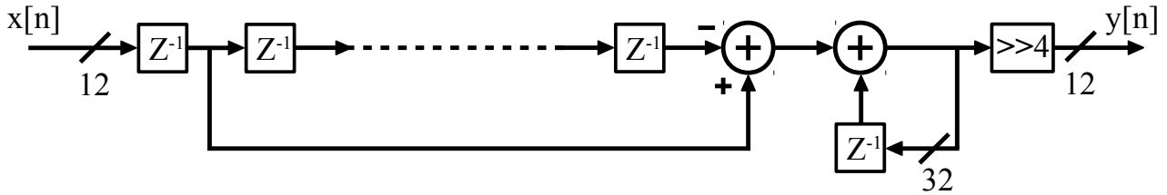
Figure 4.9: Block diagram realization of the MAF.
