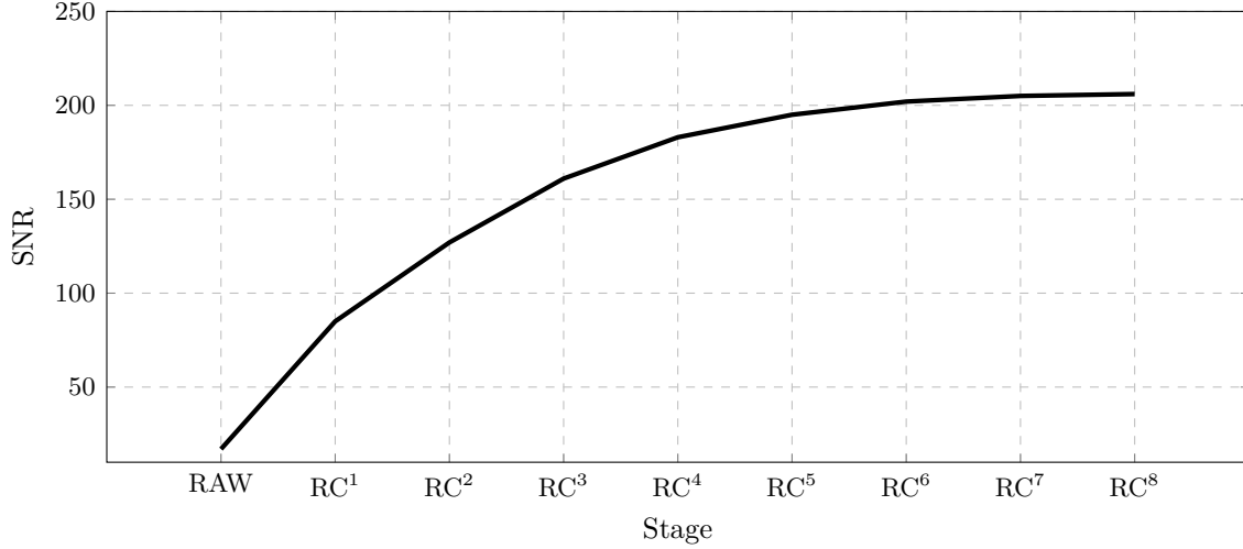
Figure 4.18: SNR as function of the RC^n stage.
