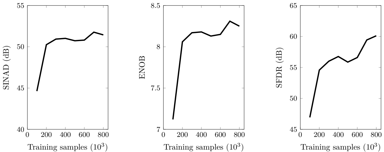
Figure 5.11: Figures of merit outcomes for different numbers of training samples using a sinusoidal signal as input.
