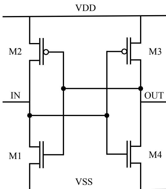
Figure 5.22: SRAM cell.
