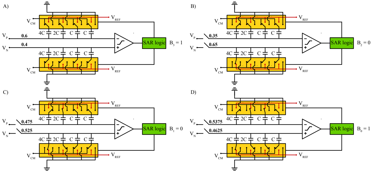
Figure 2.4: Example of a conversion of a fully differential 4-bits SAR ADC architecture.
