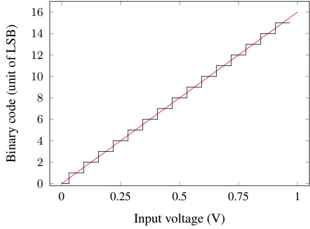
Figure 2.1: Ideal characteristics of a 4 bit ADC
