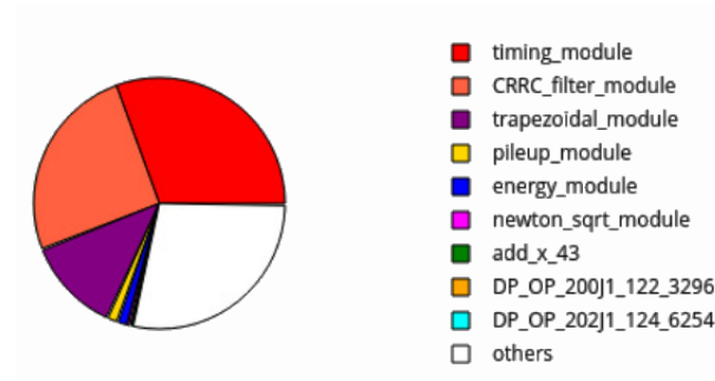
Figure 5.36: Pie chart of the power budget distribution among the sub-modules of the DSP chip.
