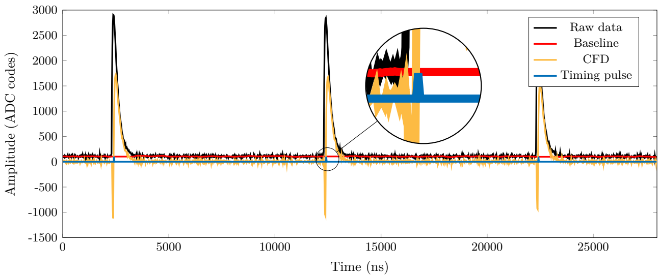
Figure 5.28: Example of CFD filtering with baseline correction and the pulse generated for signals of different amplitudes.
