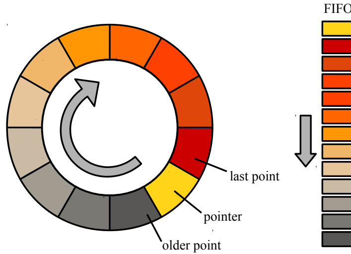
Figure 4.7: The circular buffer (on the left) and its equivalent FIFO (on the right).
