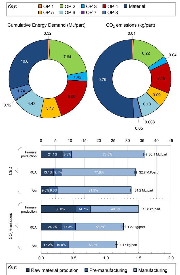
Fig. 5. Summary of the CED (left) and CO 2 emissions (right), detailing the relative shares of material consumption and electricity.
