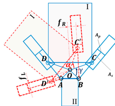
Figure A1. Steering joint kinematics: straight line (blue), turning (red).
