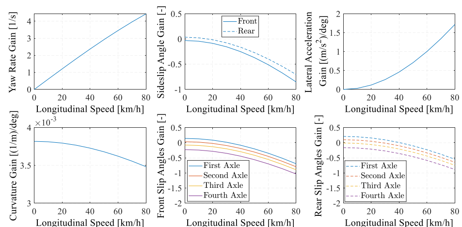
Figure 12. Steady-state gains of yaw rate (top left), front and rear sideslip angles (top central), front lateral accelerations (top right), curvatures (down left), front slip angles (down central) and rear slip angles (down right) for different front longitudinal speeds.
