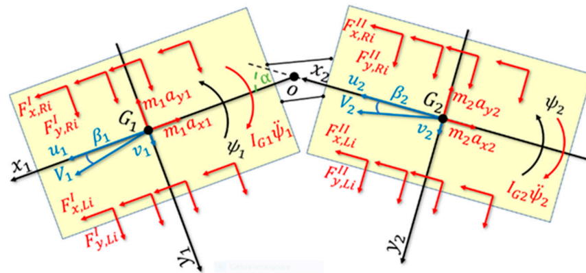
Figure 2. Free body diagram of ATV (top view). Reprinted with permission from ref. [19]. Copyright 2020 Springer Nature Switzerland AG.
