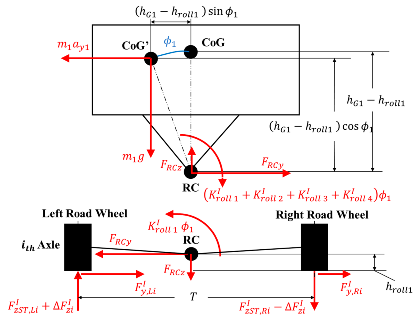
Figure 5. Free body diagram of the ATV (front unit view).
