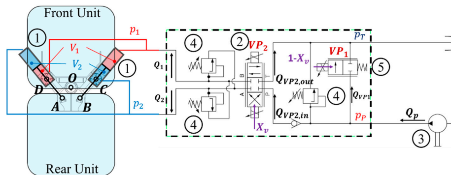
Figure 6. Hydraulic steering circuit 1—Double-acting cylinders; 2—Double-solenoid flow rate proportional valve; 3—Pump; 4—Pressure relief valves; 5—Single-solenoid flow rate proportional valve. Adapted with permission from ref. [19]. Copyright 2020 Springer Nature Switzerland.
