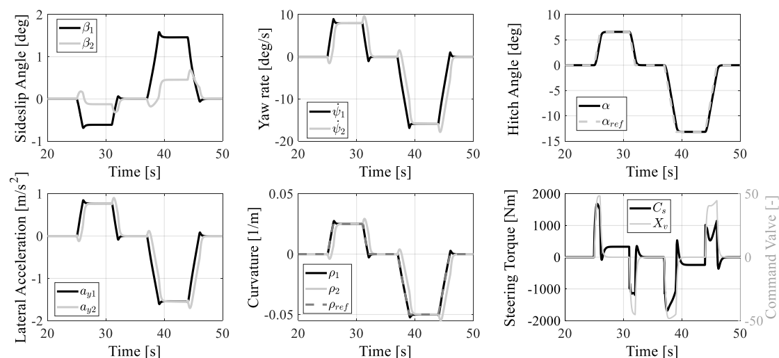
Figure 16. Sideslip angles, yaw rates, hitch angle, lateral accelerations, curvatures, steering torque, and hydraulic command valve during a multiple turn maneuver, with the hitch angle controller with SBL and fixed PID gains applied to the non-linear model at constant ATV speed u_1 = 20 km/h. Reprinted with permission from ref. [19]. Copyright 2020 Springer Nature Switzerland AG.
