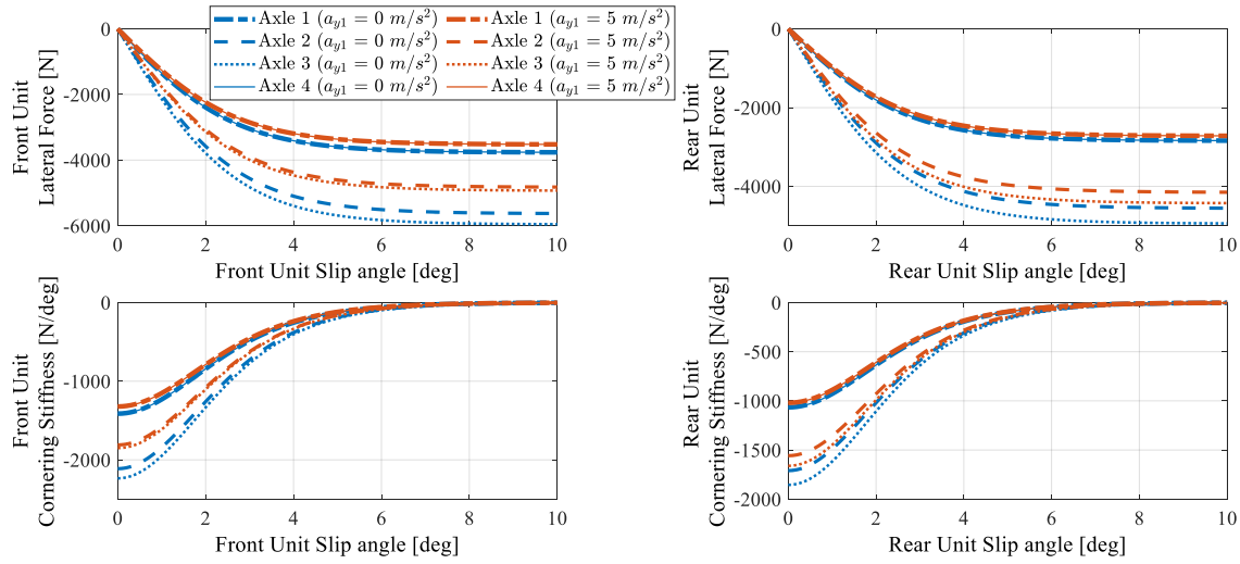
Figure 8. Front (left) and rear (right) unit axle lateral forces (top) and cornering stiffness (down) as a function of slip angles for different values of the lateral acceleration.
