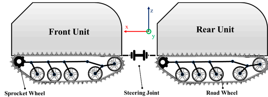
Figure 1. Simplified schematic of the articulated tracked vehicle (ATV).
