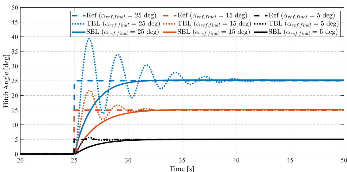
Figure 15. Step response of the non-linear ATV model with TBL and SBL at u_1 = 20 km/h.
