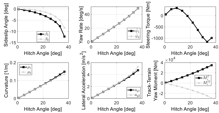
Figure 7. Sideslip angles, yaw rates, steering torque, curvatures, lateral accelerations, and track-terrain yaw moment characteristics from the non-linear model at a constant speed u_1 = 20 km/h.
