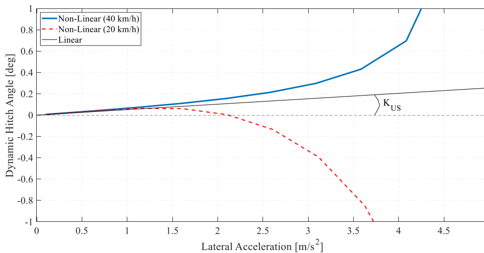
Figure 13. Understeer characteristics for the non-linear model at 40 km/h (blue solid line) and at 20 km/h (red dashed line) and for the linear model (black solid line).
