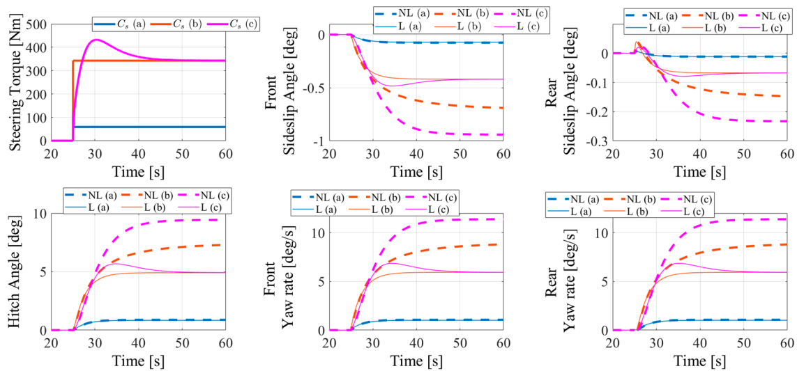
Figure 10. Non-linear (NL) and Linear (L) models response in terms of front ( \beta_1 ) and rear ( \beta_2 ) sideslip angles, hitch angle ( \alpha ), front ( \dot{\psi}_1 ) and rear ( \dot{\psi}_2 ) yaw rates for three steering input torques C_s at a constant longitudinal speed u_1 = 20 km/h.
