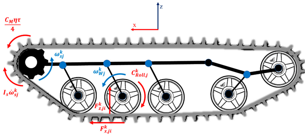
Figure 3. Free body diagram of each track rotational dynamics.
