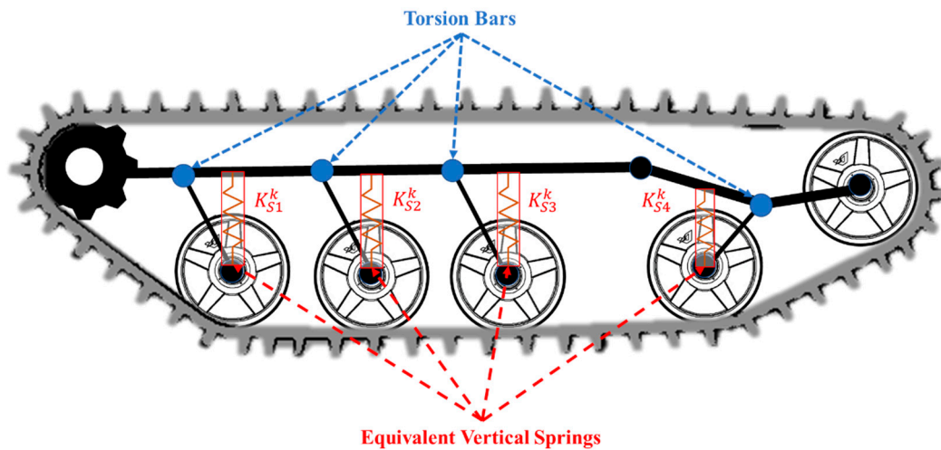
Figure 4. Simplified schematic of the ATV suspension system.
