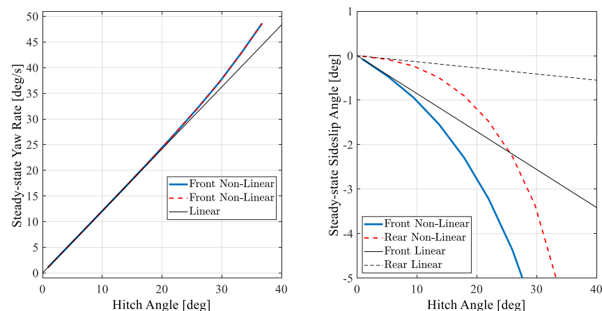
Figure 11. Steady-state yaw rate, front and rear sideslip angles characteristics for a constant longitudinal speed u_1 = 20 km/h.
