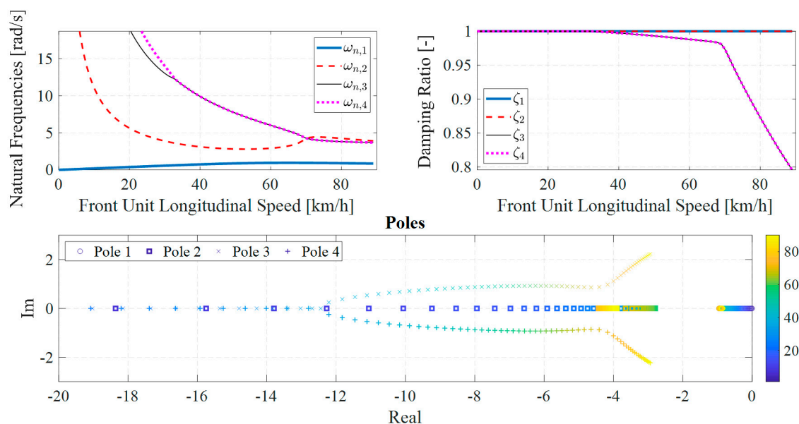
Figure 9. Natural frequencies \omega_{n,i} , damping ratio \zeta_i and poles of the ATV linear model as functions of vehicle longitudinal speed u_1 .
