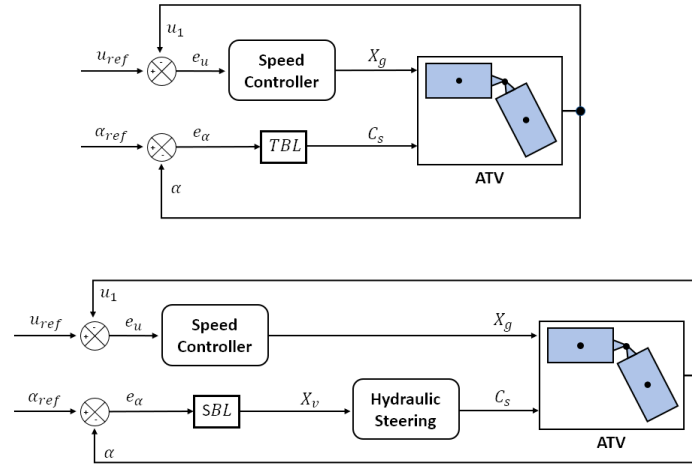
Figure 14. Simplified schematic of the Torque-Based Logic (TBL) and Speed-Based Logic (SBL) applied to the ATV non-linear model.
