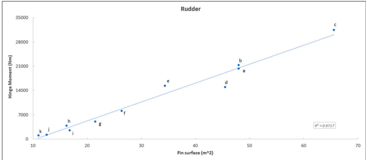
Figure 5. Surrogate model results for rudder
