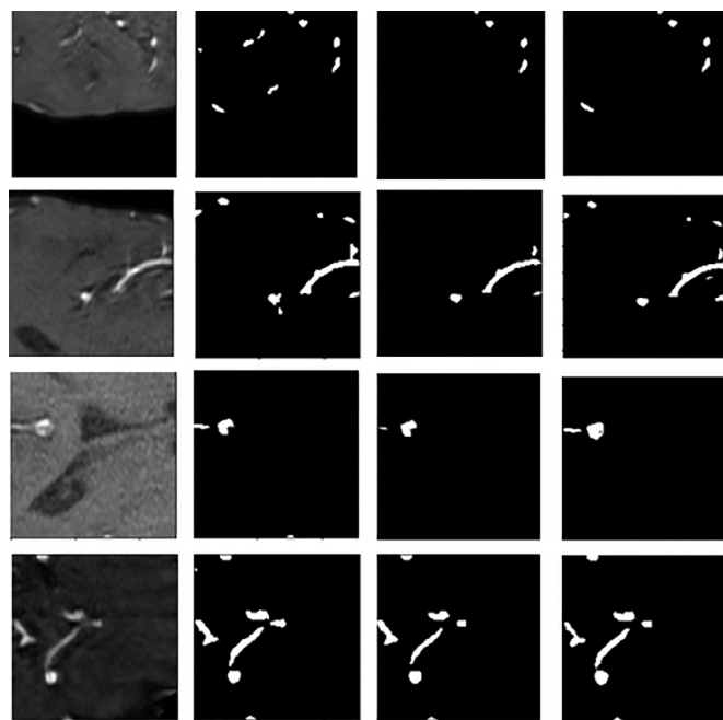
Fig. 16. Examples of the generated training set \mathcal{T}_M . From left to right original TOF image, ground truth, GMM pseudo-labels and K-means pseudo-labels.
