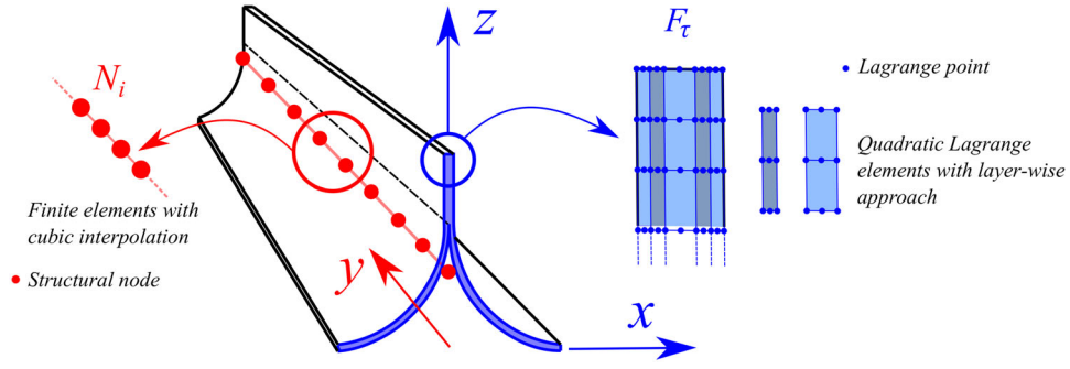
Figure 3. One-dimensional model of the TRAC.
