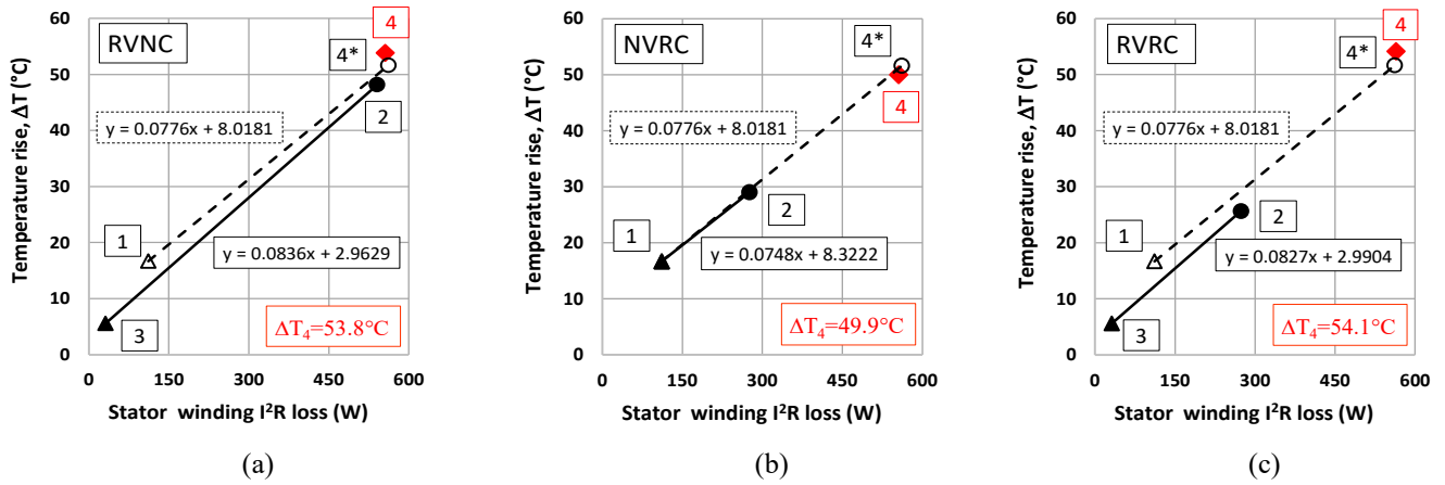
Fig. 6: Temperature rise for the tested 15kW IM for the three equivalent loading methods: (a) reduced voltage ( V_s = 0.7 V_n ) and nominal current, (b) nominal voltage and reduced current ( I_s = 0.73 I_n ), and (c) reduced voltage and reduced current ( V_s = 0.7 V_n and I_s = 0.73 I_n ).
