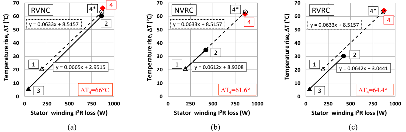
Fig. 7: Temperature rise for the tested 18.5kW IM for the three equivalent loading methods: (a) reduced voltage ( V_s = 0.7 V_n ) and nominal current, (b) nominal voltage and reduced current ( I_s = 0.73 I_n ), and (c) reduced voltage and reduced current ( V_s = 0.7 V_n and I_s = 0.73 I_n ).
