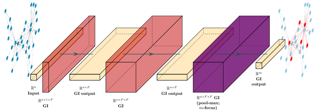
Figure 5. Example of a GINN archetype with depth H = 2 and max-pooling operation for the output layer. The output matrices Y of the NN layers are in orange, the weight tensors W of the hidden GI layers are in red (see Definition 3), and the weight tensor W of the output GI layer with max-pooling and masking operations (see Section 2.3) are in purple.
