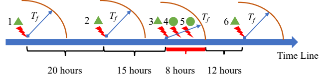
Fig. 4. Visual representation of the repetitive fault grouping procedure.
