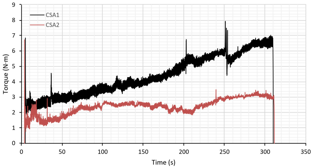
Fig. 7. Measurement of the torque on the disk during the dynamic adhesion test on clay A.
