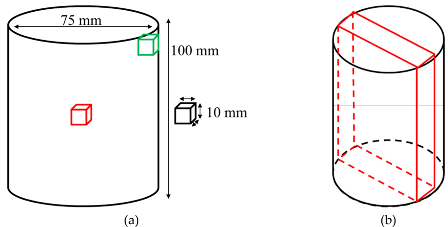
Figure 3. (a) Scheme of the can and cube dimensions, both after HIP, for study B. Additionally, the can microstructural analysis areas were pointed out, in red and green, for study A. (b) Extracted can slice for hardness mapping, study A.
