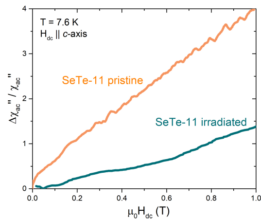
Figure 6. Fractional shift of the imaginary part of the AC susceptibility, \Delta\chi''_{ac}/\chi''_{ac} = [\chi''_{ac}(H) - \chi''_{ac}(0)]/\chi''_{ac}(0) , as a function of the applied DC magnetic field, for a pristine SeTe-11 crystal and for a SeTe-11 crystal after irradiation with 320-MeV Au ions at the fluence of 10^{11} cm ^{-2} . Data were measured at a fixed temperature of T = 7.6 K, with the field applied parallel to the c -axis and to the columnar defects induced by irradiation.
