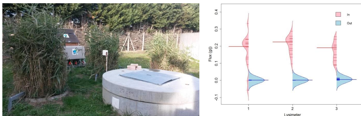
Figure 6: The three lysimeters containing the three soils studied (left); Phosphate fluxes measured at the inlet and outlet of the three lysimeters (right)
