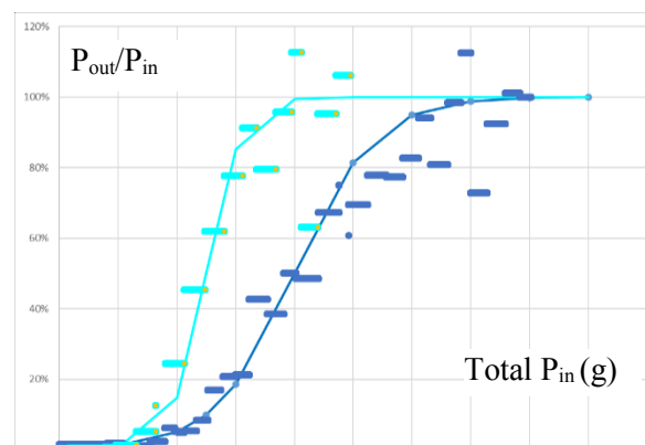
Figure 1: P break through curves trough pure (light blue) or iron-enriched (dark blue) alumina.
