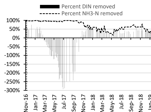
Figure 2. Percent DIN and NH 3 -N removal
