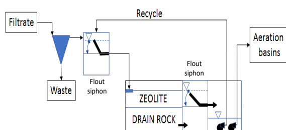
Figure 1. Section flow schematic
