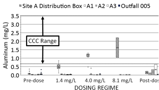
Figure 2. Total Al concentrations at Site A. Inflow is the distribution box.
