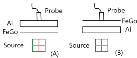
Fig. 7. Set-up configurations
