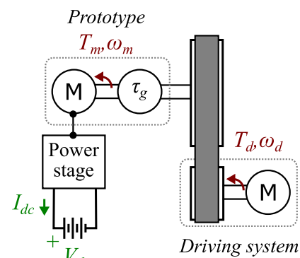
Figure 9. Scheme of the rotary electromechanical damper prototype test bed.
