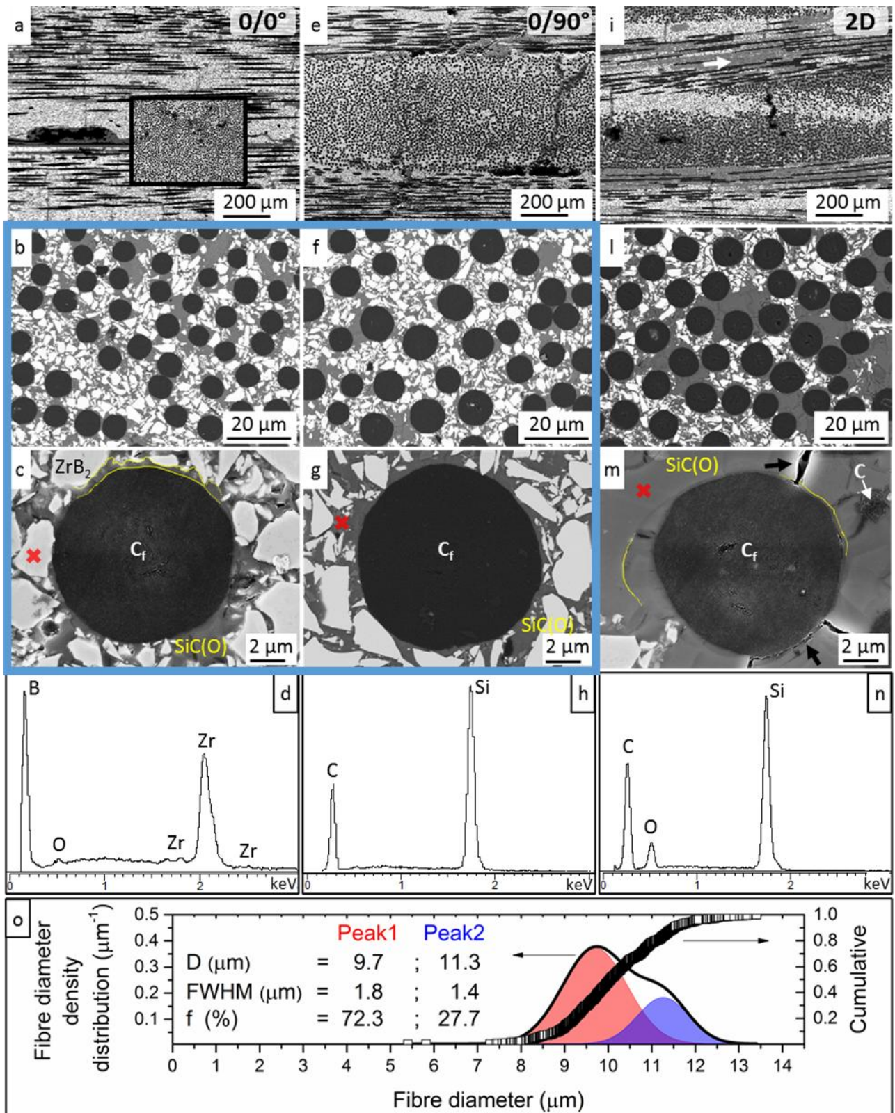
Fig. 3. Polished sections of C_f/ZrB_2-SiC composites obtained after 6 cycles of PIP. Low magnification micrographs of a) 0/0° sample, e) 0/90° sample and i) 2D sample; white arrow points a higher content of SiC(O) in intra-bundle regions. Details of microstructure of b) 0/0° sample, f) 0/90° sample, l) 2D sample. A single fibre surrounded by the matrix: c) ZrB_2 -rich area in 0/0° sample, where a SiC(O) film around the C_f is shown (a part is indicated as a yellow area), g) ZrB_2 -rich area in 0/90°, m) SiC(O)-rich area in 2D sample; yellow lines show the layered structure of SiC(O) due to repetitive PIP cycles, black arrows point cracks in SiC(O) and detachment between fibre and SiC(O) due to the shrinkage of preceramic polymer during
