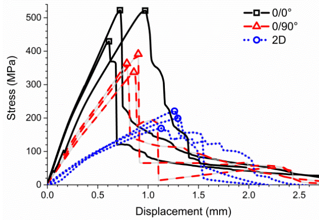
Fig. 5 Stress/displacement curves of 0/0° and 0/90° samples tested by 3-point bending, and 2D samples tested by 4-point bending. The point at the maximum stress was highlighted with a symbol.
