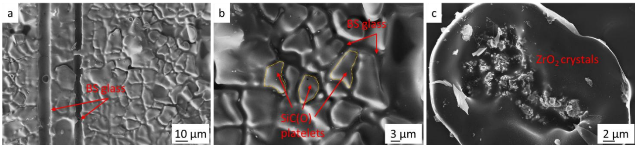
22 Fig. 6. Features of the sample surface oxidized at 1650 °C showing self-healing effects. a) Fibre evaporation 23 and voids partially filled by the BS glassy phase (BS=borosilicate), b) magnified view showing the BS glass 24 flowing in the grooves left by the SiC(O) phase, c) bubble with tiny zirconia crystals. 25 26
