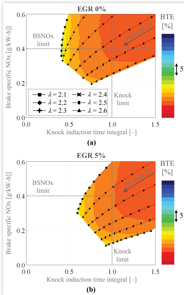
FIGURE 10 BTE obtained with different combinations of ST and lambda as a function of KITI and BSNOx for the operating point 3500 RPM × 8 bar BMEP (a) EGR 0% and (b) EGR 5%.
