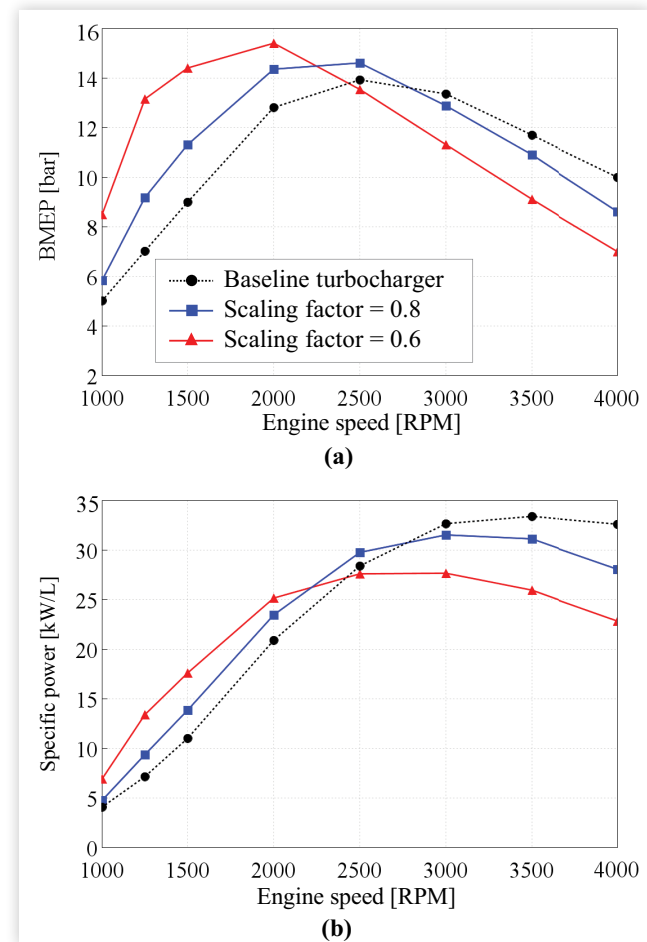
FIGURE 13 (a) BMEP and (b) specific power obtained at full load with a lambda of 2.3 and EGR 0% for different levels of SF.
