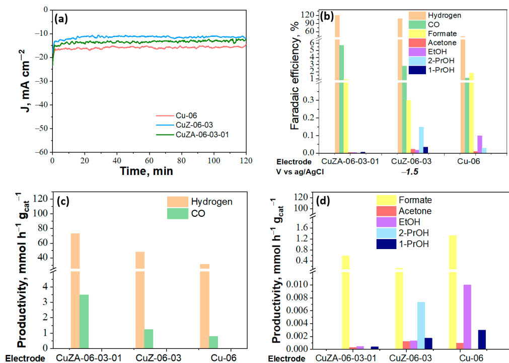
Figure 5. Chronoamperometry responses (a), Faradaic efficiencies (FEs) (b), productivities of gas (c) and liquid (d) products for CuZA-06-03-01, CuZ-06-03 and Cu-06 catalysts ( \sim 4 mg cm -2 ) with 30% of Nafion tested in 1M KHCO 3 aqueous electrolyte at -1.5 V vs. Ag/AgCl.
