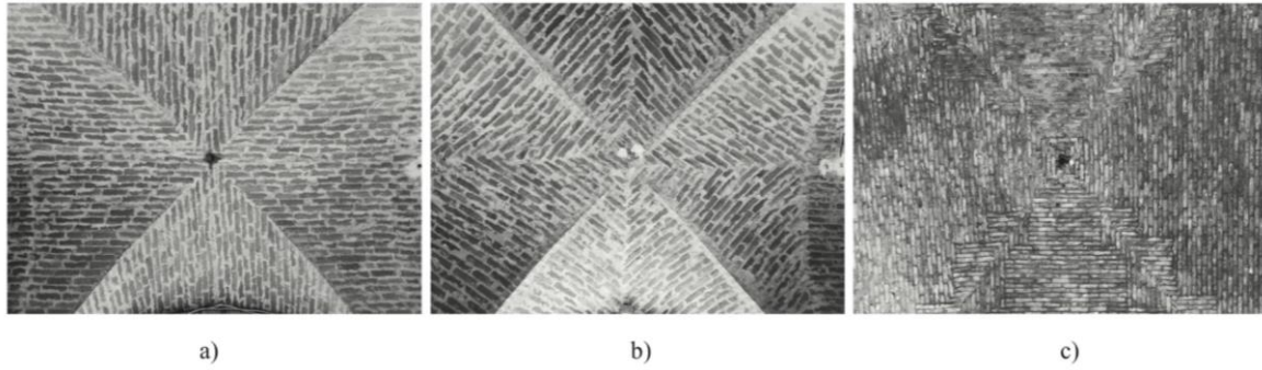
2 Figure 1: possible brick pattern in real cross vaults: radial (a), diagonal (b), pitched (c). Portico of the Palazzata 3 in Vicoforte (a, b) and Palazzo della Pilotta in Parma (c)
