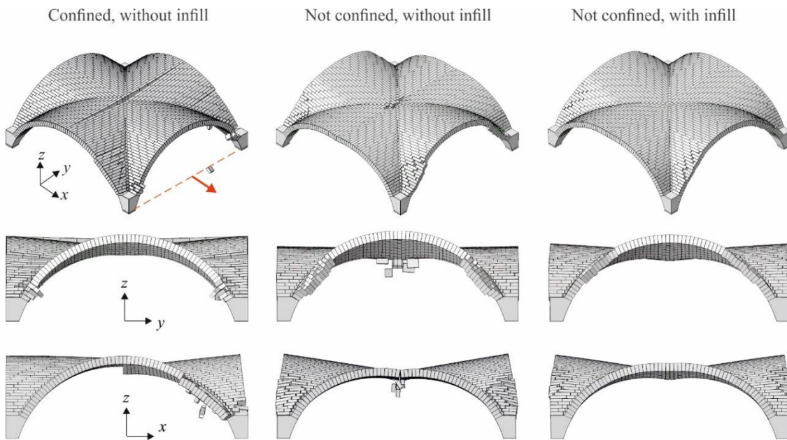
10 Figure 24: Deformed shapes for opening settlement: axonometric view (first row), y-z plane view (second row), x-z 11 plane view (third row).
