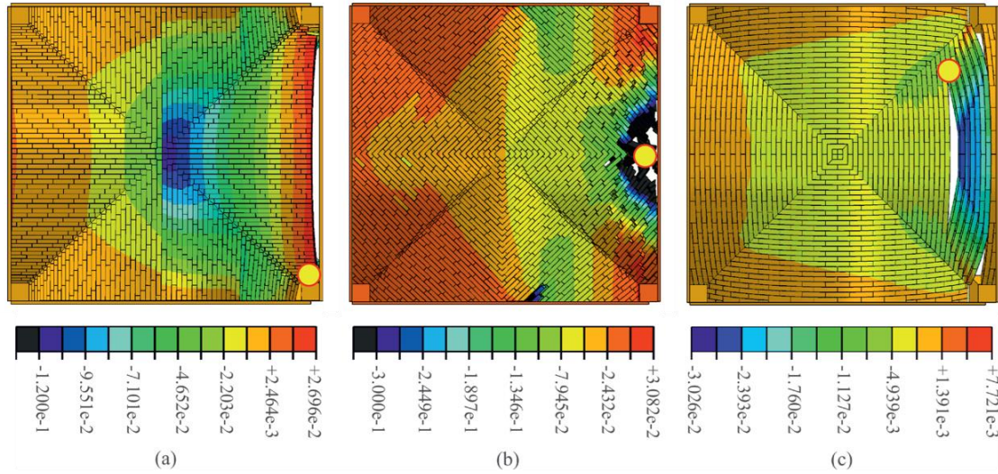
2 Figure 12: contour plot of u_z displacement [m] corresponding to an imposed opening settlement u_x/L=3.3\% for 3 radial (a), diagonal (b) and pitched (c) pattern. Yellow circles refer to the monitored control nodes.
