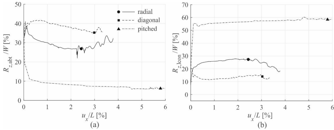
4 5 Figure 15: Reaction forces R_{z,abt} at the moving abutments (a) and R_{z,lcon} at the lateral rigid boundaries (b) versus 6 normalized imposed displacement for opening settlement
