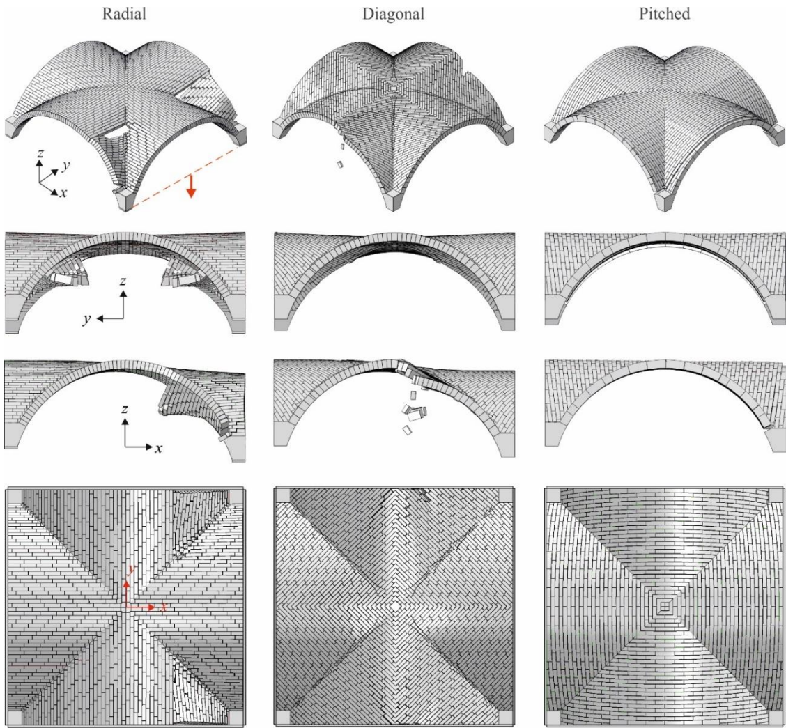
Figure 16: Deformed shapes for vertical settlement: axonometric view (first row), y-z plane view (second row), x-z plane view (third row) and plan view (fourth row).
