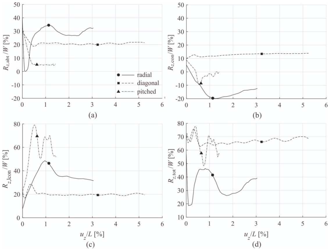
19 Figure 18: Vertical reaction forces R_{z,abt} at the moving abutments (a), R_{z,con} against moving boundary (b), R_{z,lcon} 20 along lateral rigid boundaries (c) and total reaction force R_{z,tot} (d) versus normalized imposed displacement for vertical 21 settlement
