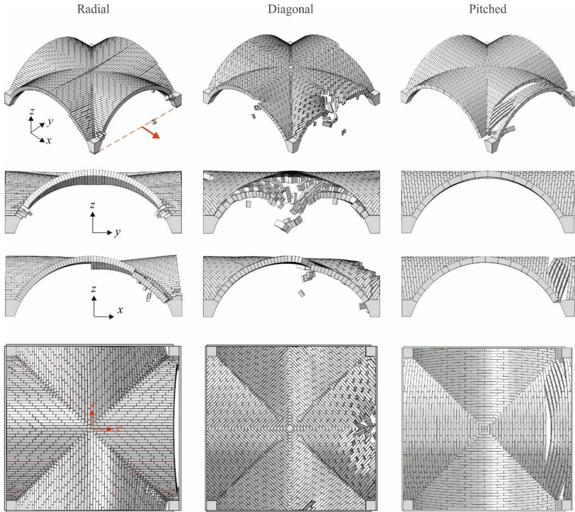
7 8 Figure 11: Deformed shapes for opening settlement: axonometric view (first row), y - z plane view (second row), x - z 9 plane view (third row) and plan view (fourth row).
