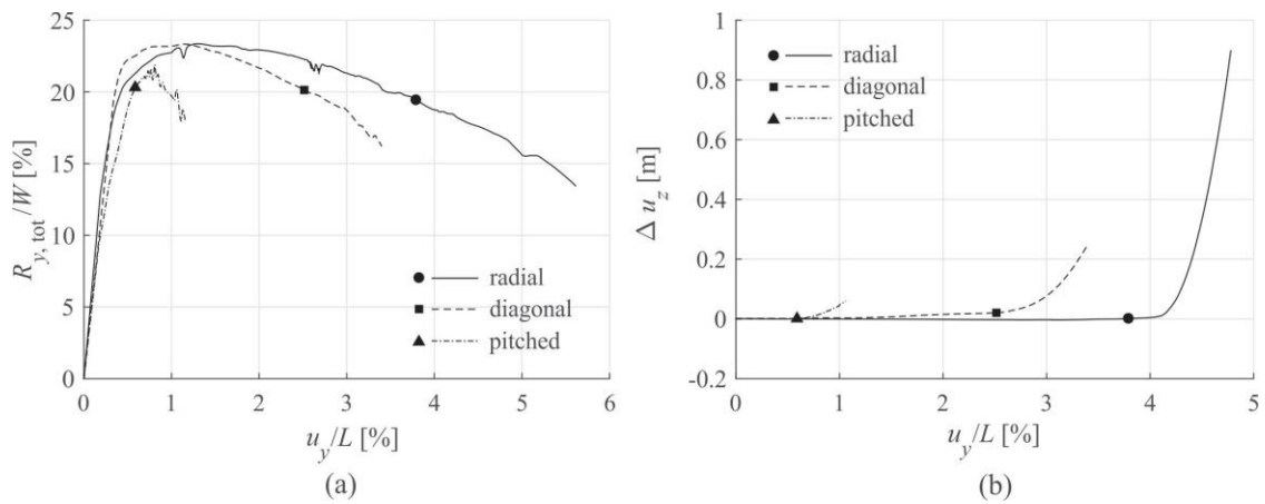
18 Figure 23: Total R_y reaction force versus imposed displacement (a) and differential vertical displacement versus 19 normalized imposed displacement (b) for shear displacement.
