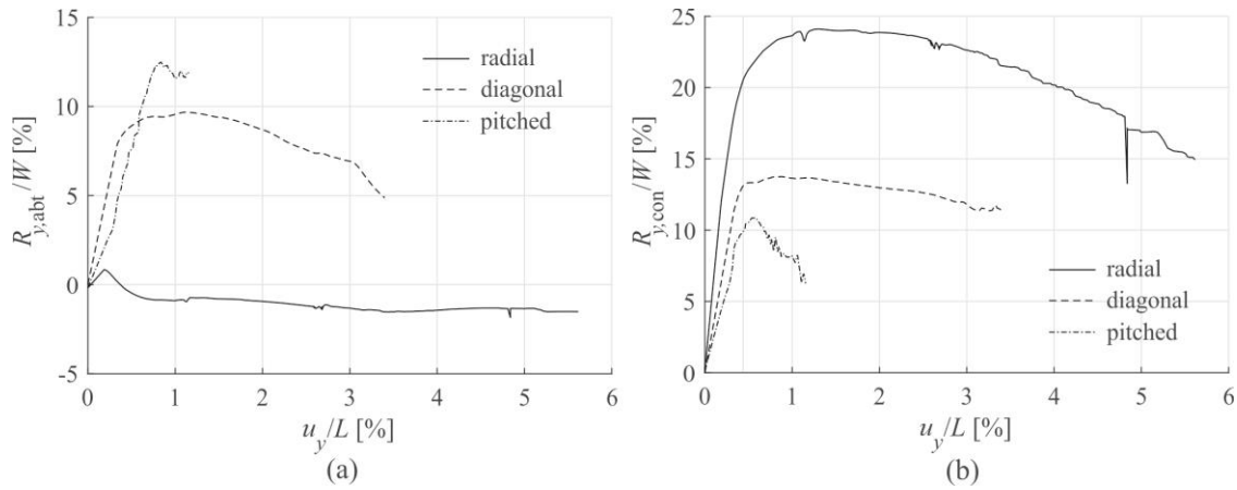
15 Figure 22: Reaction force R_{y,abt} at the abutments of the vault (a) and R_{y,con} of the deformable arches (b) versus 16 normalized imposed displacement for shear displacement.
