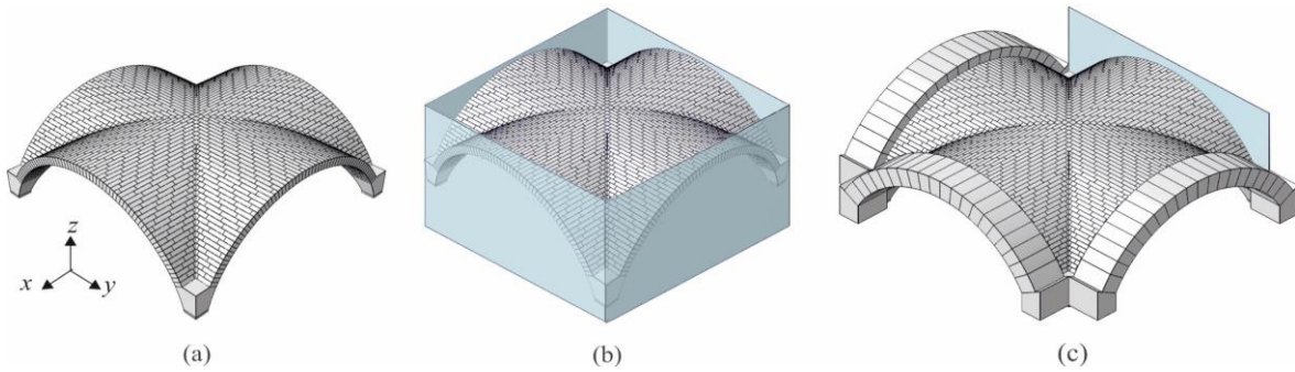
8 (a) (b) (c) 9 Figure 6: no confinement (NC) (a), rigid lateral confinement (RC) (b) and boundary deformable arches (DA) (c)
