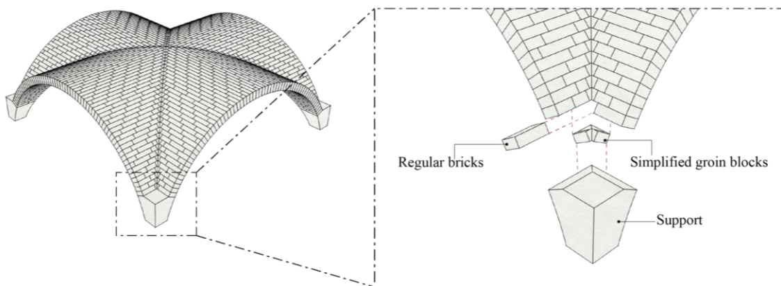
23 24 Figure 2: Discretization of the vault's geometry
