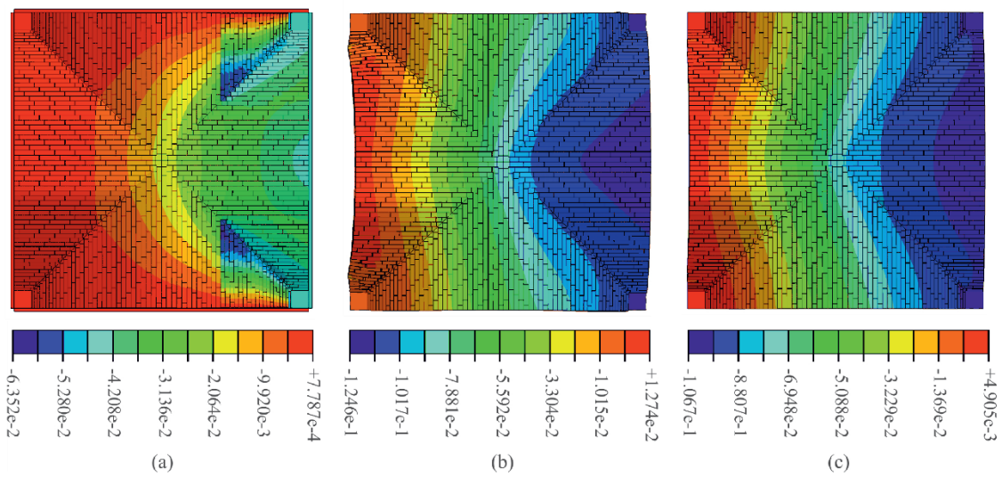
6 7 Figure 28: contour plot of u_z displacement [m] corresponding to an imposed vertical settlement u_z/L= 3.23\% for 8 confined vault without infill (a), not confined vault without infill (b) and with infill (c)
