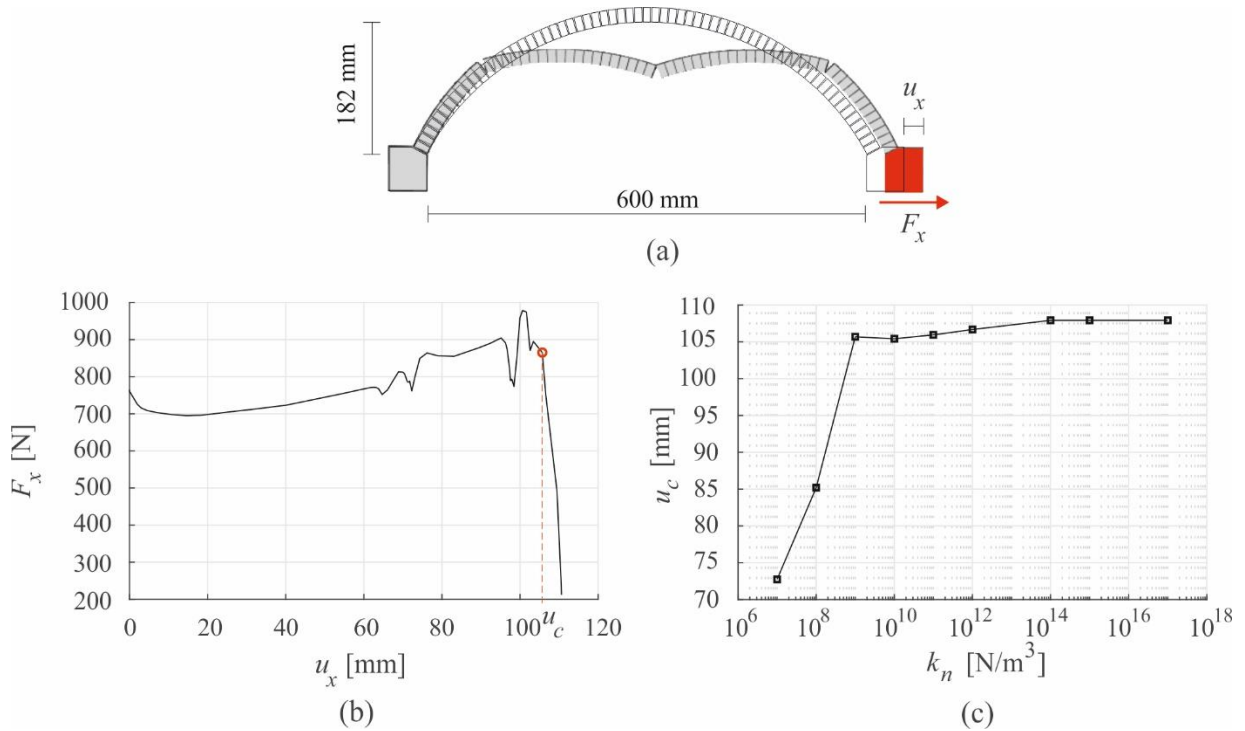
10 Figure 3: scheme of the arch with imposed settlement u_x (a), load-displacement curve for k_n = 5 \cdot 10^9 \text{ N/m}^3 (b) and 11 displacement u_c at collapse versus k_n (c).
