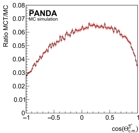
Fig. 13 Ratio of the \cos(\Theta) distributions in the c.m. frame for the final selected \Xi^+_{c.m.} candidates in the process \bar{p}p \rightarrow \Xi^+ \Lambda K^- . MC indicates the generated candidates and MCT the MC truth partners of the final selected candidates
