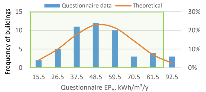
Fig. 6. Normal distribution for space heating considering the class of buildings with 0.25 < S/V < 0.45 \text{ m}^{-1} and 1972 < PC < 1981 (validated with \chi^2 and KS tests). Green lines represent the right range “average \pm 2 times the st. deviation”.
