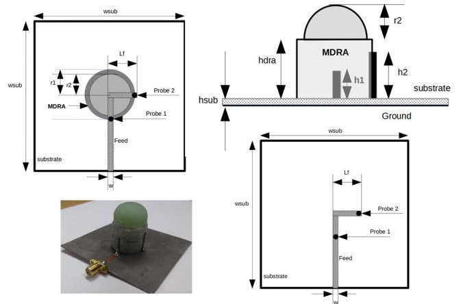
Fig. 1: Geometry of MDRA and fabricated prototype
