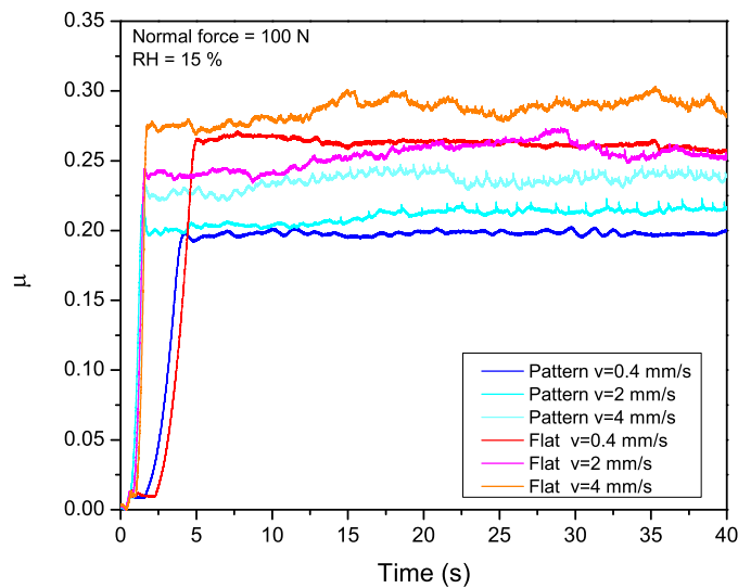
Fig. 11: Comparison of the time evolution of the friction coefficient for the nominally flat and patterned cases, with F = 100 N, RH=15%.
