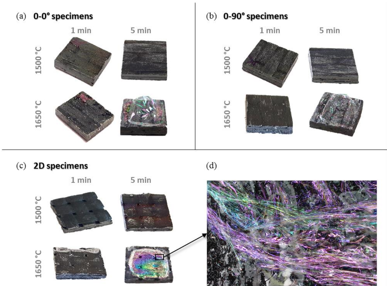
Figure 4. Appearance of the oxidized specimens after bottom loading furnace tests at 1500 and 1650 °C for 1 and 5 min in air: (a) sample 0-0°, (b) sample 0-90° and (c) sample 2D. (d) Optical image detail of a soft iridescent glass bubble grown on the surface of the specimen shown in (c).
