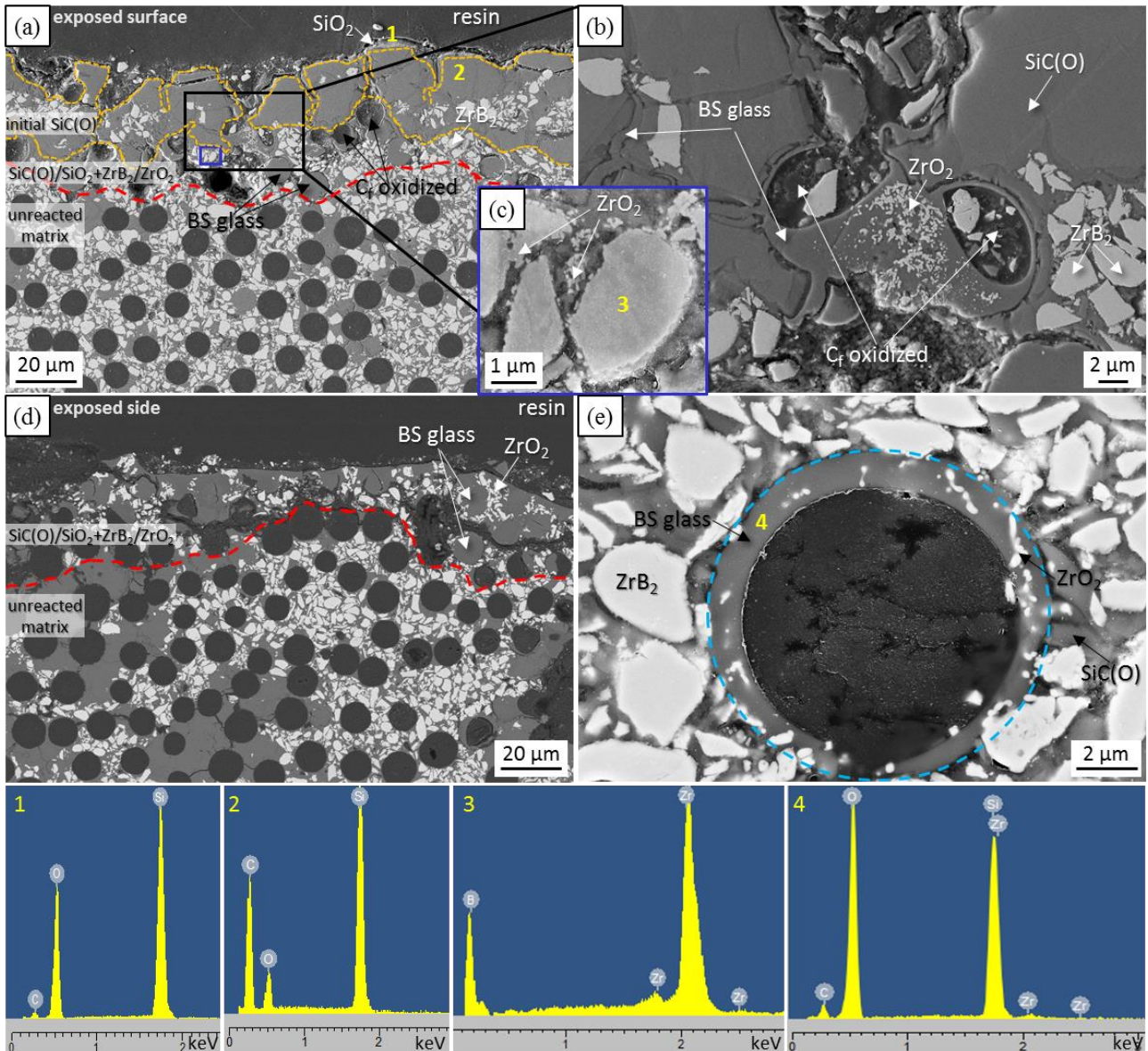
Figure 7. Polished cross section of the specimen (sample 0-0°) after short term oxidation test at 1500 °C for 1 min in air. (a) Micrograph of the exposed surface, SiC(O)-rich area, (b) magnification of the BS glass in the voids left by the C f oxidation and (c) magnification of the partially oxidized ZrB 2 particles; (d) micrograph of the exposed side. (e) High magnification micrograph of a fibre where the oxidation stopped thanks to the BS glass (marked with blue circle) that surrounded it. In the bottom EDS spectra of the phases as numbered.
