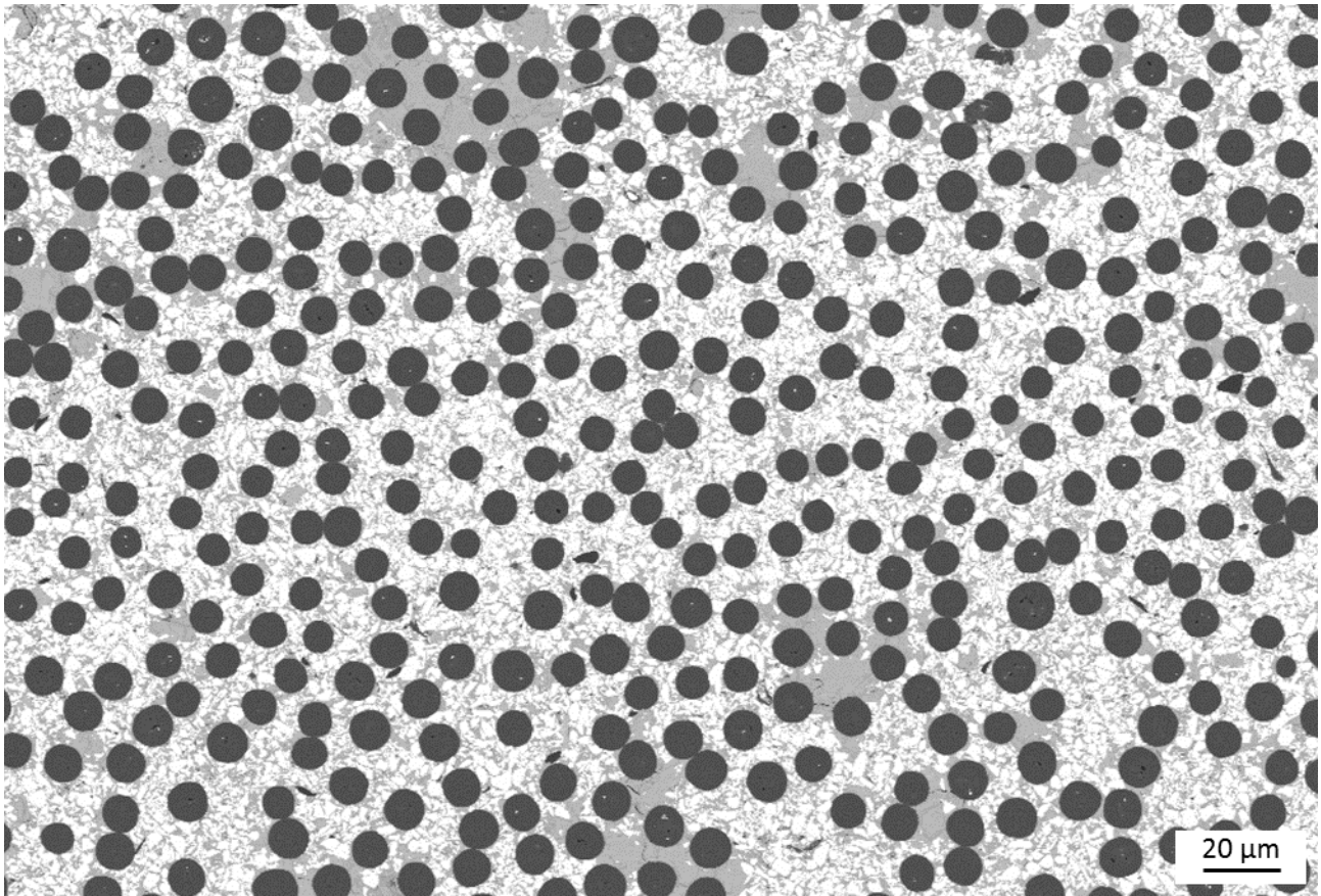
Figure 2. SEM micrograph of the polished section of the 0-0° sample, showing the good homogeneity of carbon fibre (black phase) embedded in ZrB_2 (white phase) – SiC (grey phase) matrix.
