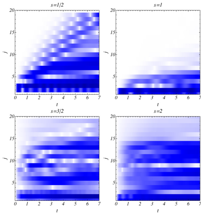
FIG. 3. Time evolution of \langle S_z(j,t) \rangle - \langle S_z(j,0) \rangle after switching on a local field, 5S_z(j_0) : (a) on j_0 = 2 of a spin s = 1/2 chain, (b) on j_0 = 1 of a spin s = 1 chain, (c) on j_0 = 2 of a spin s = 3/2 chain, and (d) on j_0 = 1 of a spin s = 2 chain. The light cones are absent for s = 3/2 and s = 2 .
