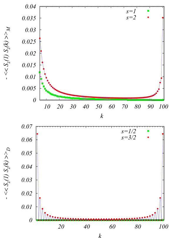
FIG. 2. Connected correlation functions, -\langle \langle S_z(1) S_z(k) \rangle \rangle , as a function of k for integer (top, for 5 \leq k \leq L ), and half-integer (bottom, for 2 \leq k \leq L ) spins for chains of length L = 100 .
