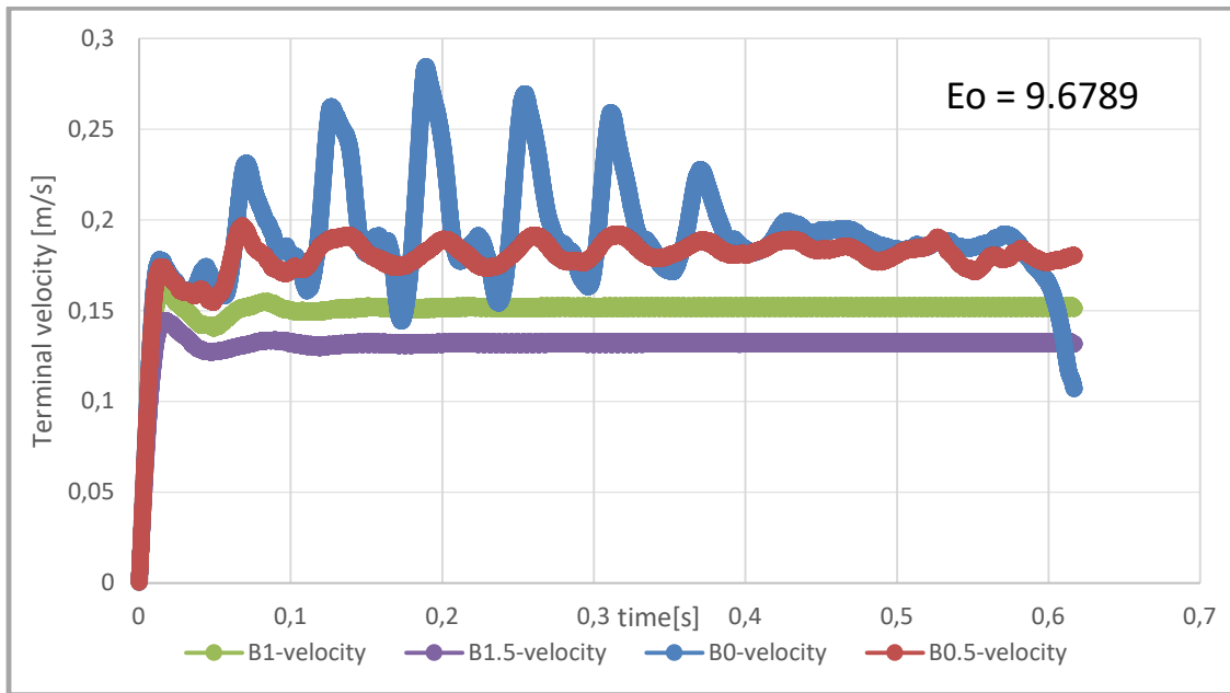
Figure 58 "Velocity vs time for different external magnetic field B."
