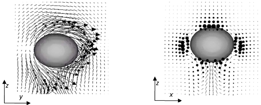
Figure 38 "Left: y-z section of current density J. Right: x-z section of J, D= 1.2mm."
