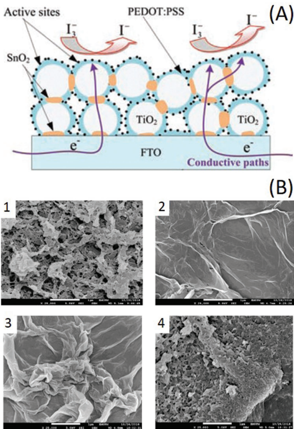
Figure 10. A) Microstructured model for PEDOT:PSS/TiO 2 /SnO 2 composite, highlighting the good adhesion to the FTO and the electron path. B) FESEM images of 1) pristine PEDOT, 2) pristine rGO, 3) PEDOT-rGO, and 4) PEDOT-rGO/Al 2 O 3 . Reproduced with permission. [273,277] Copyright 2016, American Scientific Publishers. Copyright 2019, Elsevier.
