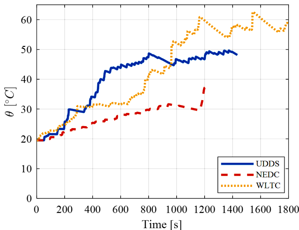
Figure 22. The temperature of the 14s12p battery pack on different driving cycles.
