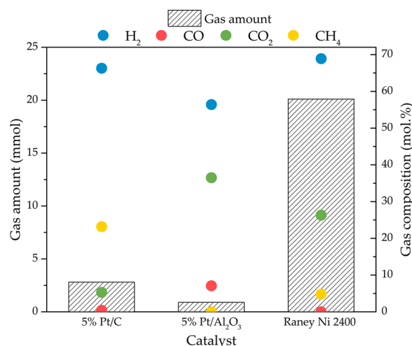
Fig. 2. APR of wheat straw hydrolysate with different catalysts. Reaction conditions: 250 °C, 2 h, 50 mL hydrolysate (data from [32]).
