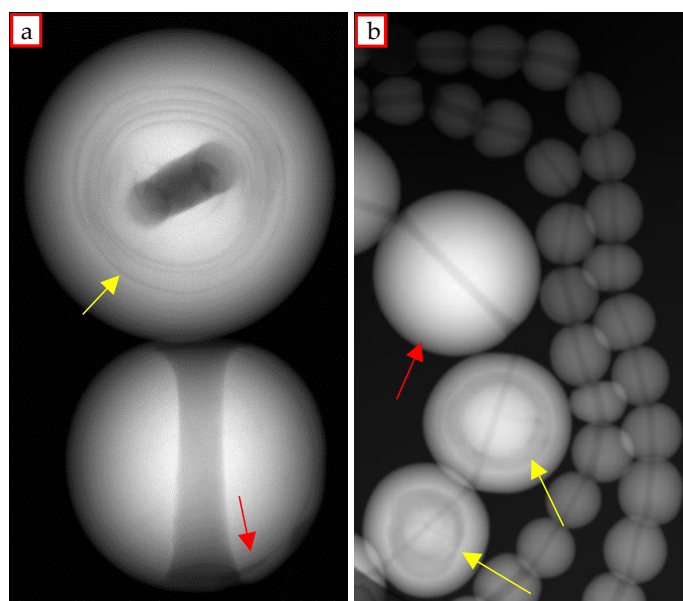
Figure 1. Radiographic images of (a) natural pearl and beaded cultured pearl and (b) a detail of a necklace in which both natural and cultured pearls could be distinguish (yellow arrows: alternated aragonite and conchiolin layers, characteristic of natural pearls; red arrows: organic layer typical of cultivated pearls).
