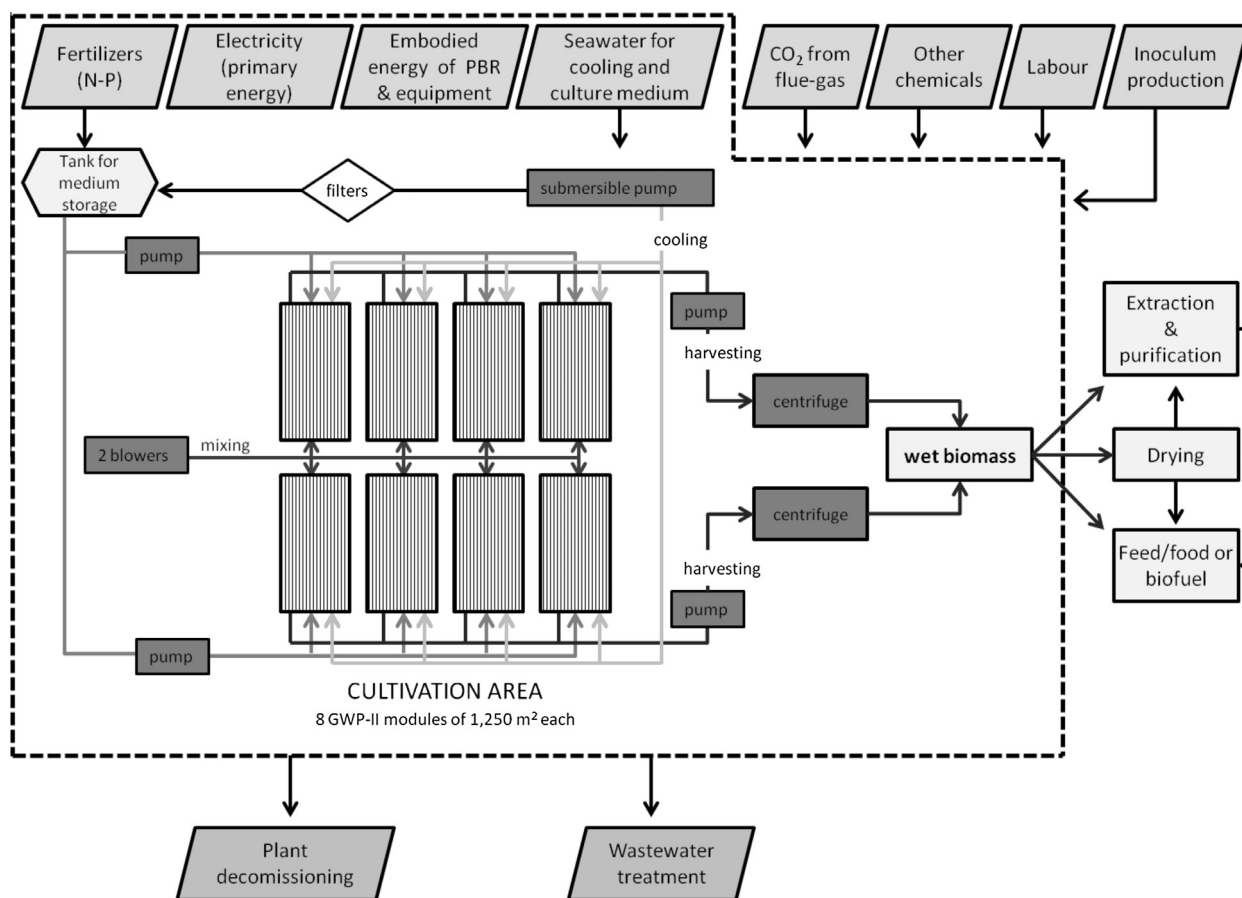
Fig. 1. Scheme of algal biomass production and downstream processes. Boundary limits (dotted box) for the energy analysis are shown.
