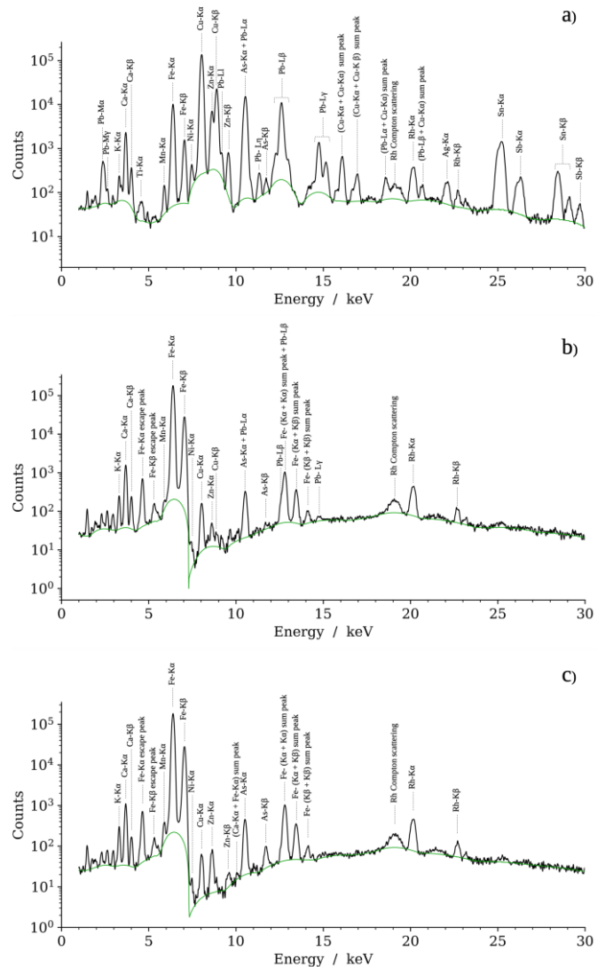
Figure 4. XRF spectra collected on the two turnbuckles: nut of Turnbuckle1 (a), one of rods on Turnbuckle1 (b), nut of Turnbuckle 2 (c). The black line is the acquired spectrum, while the computed baseline is in green.
