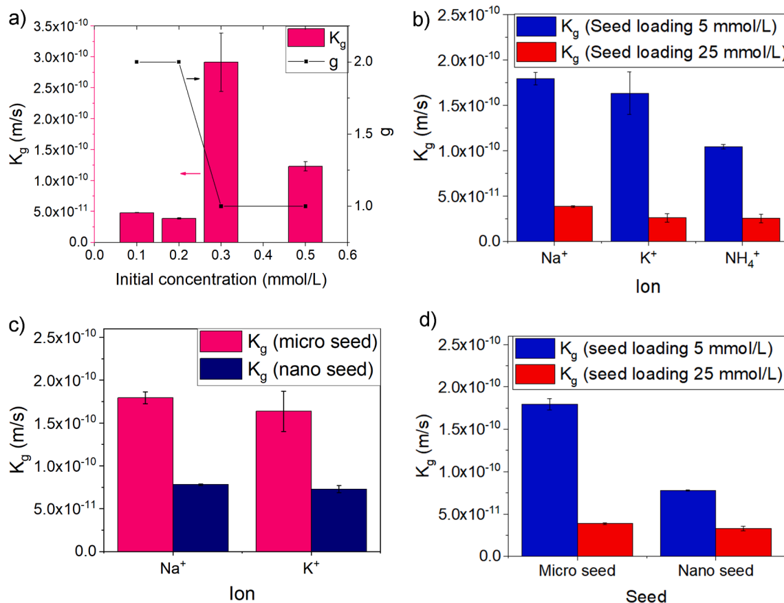
Fig. 5. Operating parameters effects on the CaCO 3 growth kinetics. a) Ion and Ca 2+ and CO 3 2- concentration effect (Constant micro seed loading equal to 5 mmol/kg, Na 2 CO 3 as CO 3 2- source). b) Ion and micro seed loading effect (Constant Ca 2+ and CO 3 2- concentration, 0.2 mM). c) Seed size and CO 3 2- source influence (Constant Ca 2+ and CO 3 2- concentration, 0.2 mM and seed loading equal to 5 mmol/kg). d) Seed size and loading (Constant Ca 2+ and CO 3 2- concentration, 0.2 mM; Na 2 CO 3 as CO 3 2- source).
